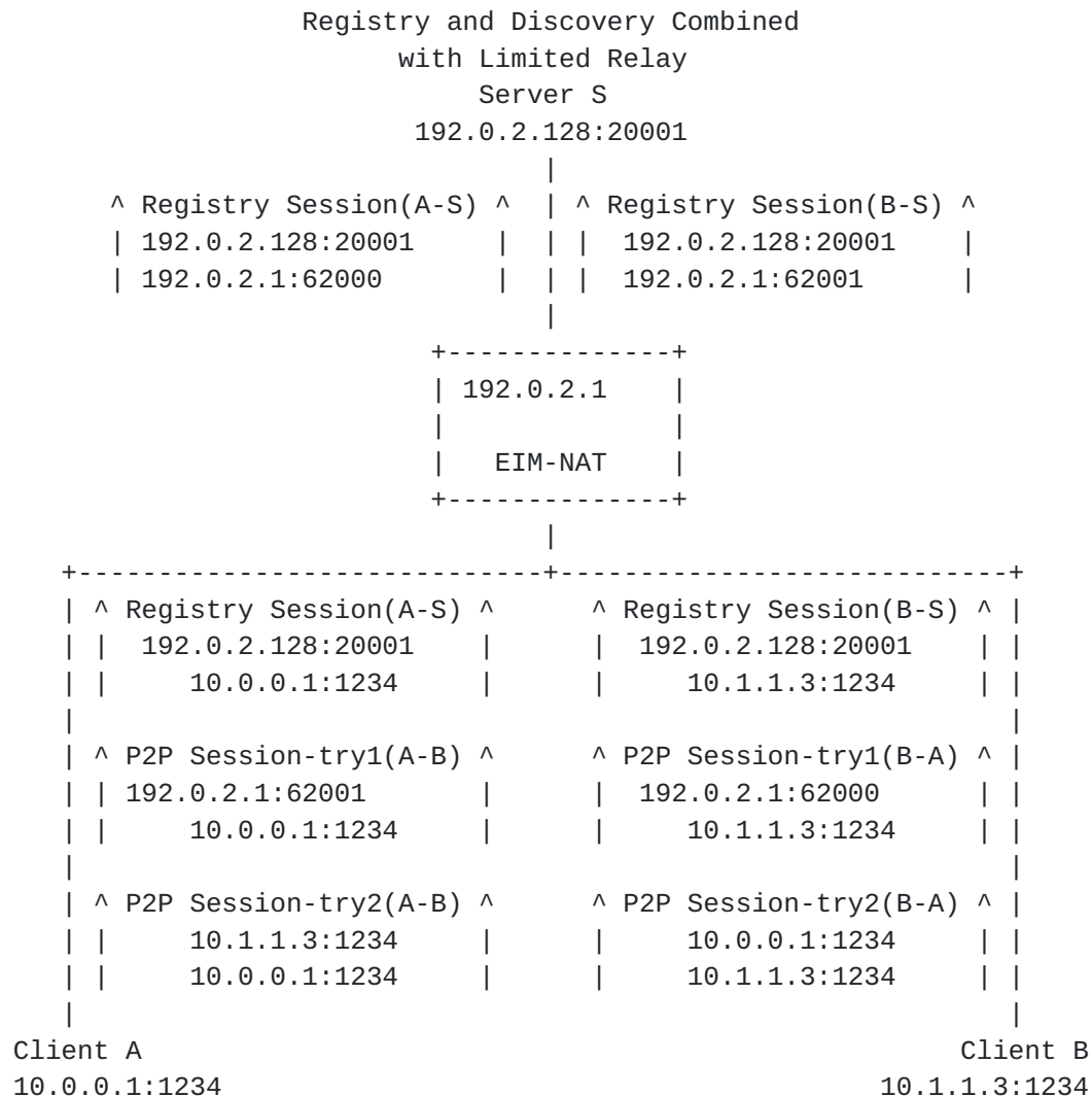
Figure 4: Use of local and public endpoints to communicate with peers
