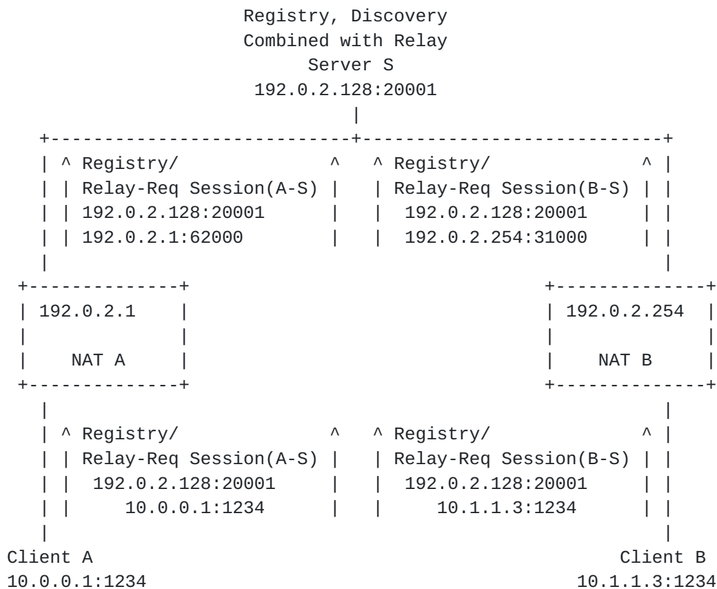
Figure 1: Use of a Relay Server to communicate with peers
