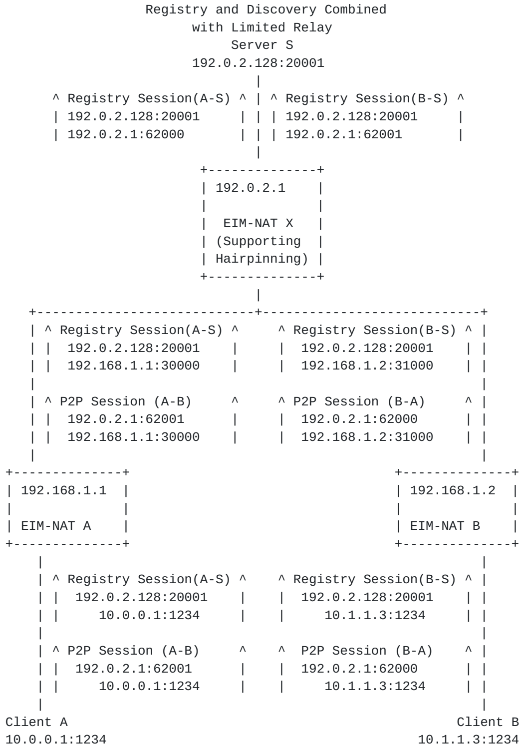
Figure 5: Use of Hairpinning in setting up direct communication
