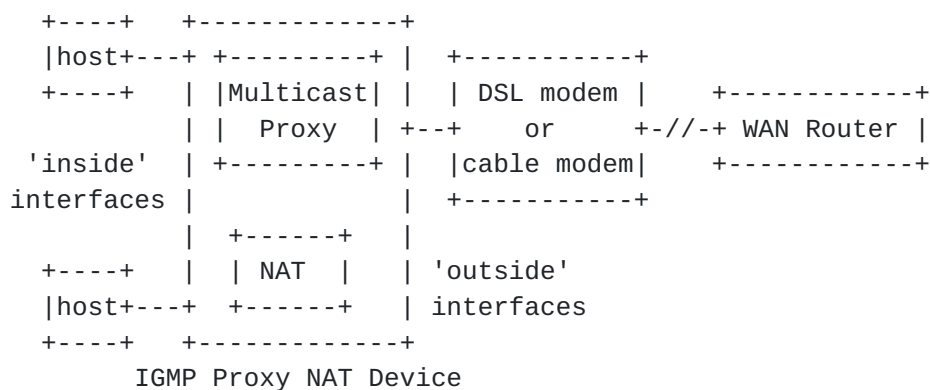
Figure 2: Network with NATing IGMP Proxy
