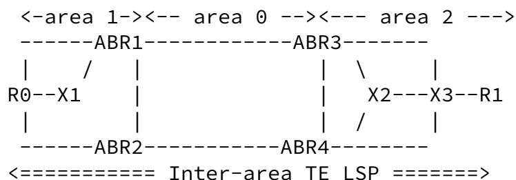
Figure 1 - Example of topology for the inter-area TE case
