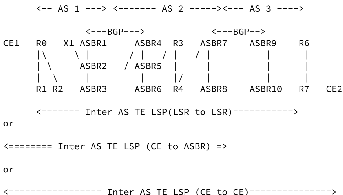
Figure 2 - Example of topology for the inter-AS TE case
