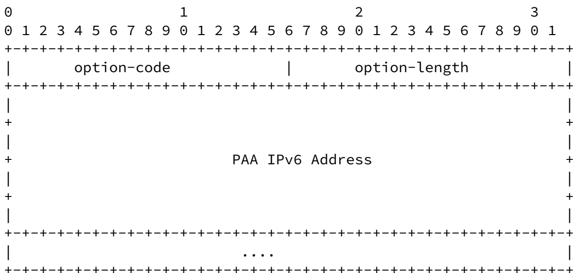
Figure 2: PAA DHCPv6 option
