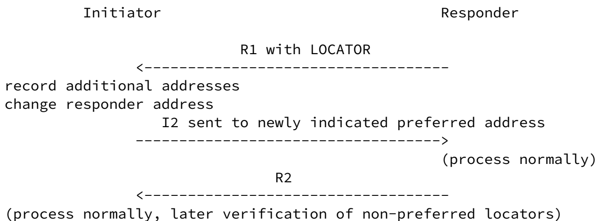
Figure 7: LOCATOR Inclusion in R1
