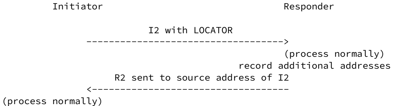
Figure 8: LOCATOR Inclusion in I2
