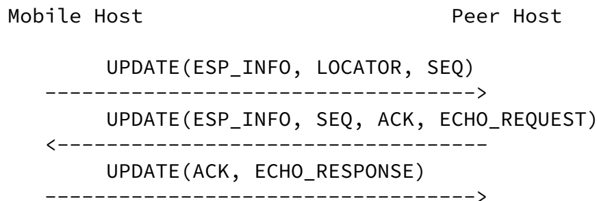
Figure 3: Readdress without Rekeying, but with Address Check
