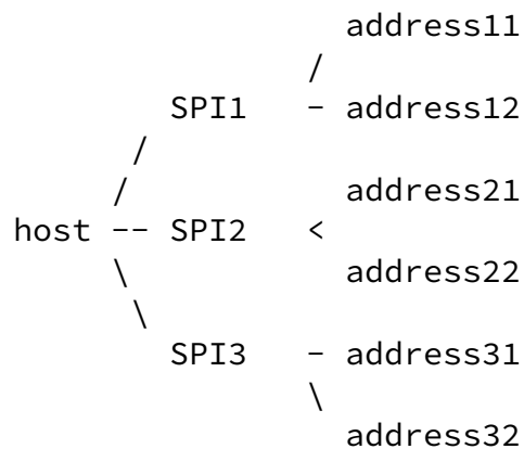
Figure 11: Relation between Hosts, SPIs, and Addresses (General Case)
