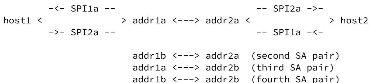
Figure 6: Dual Multihoming Case in Which Each Host Uses LOCATOR to Add a Second Address
