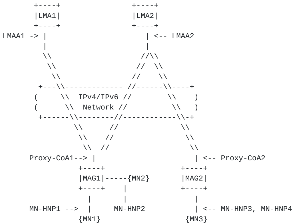
Figure 1: Proxy Mobile IPv6 Domain
