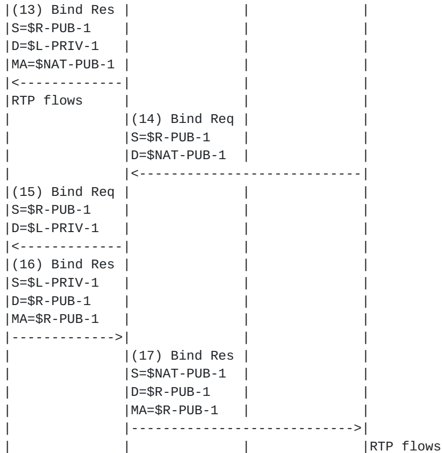
Figure 9: Example Flow
