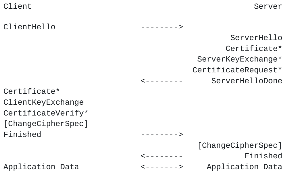
Figure 1. Message flow for a full handshake
