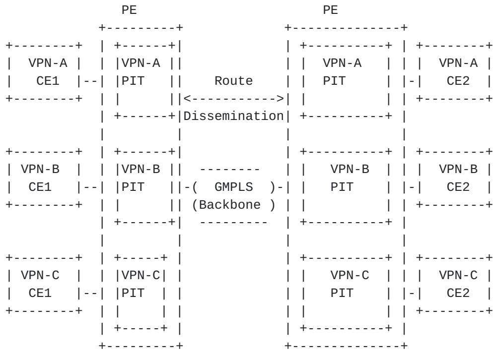
Figure 3: Basic Mode L1VPN Service
