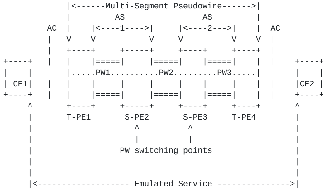
Figure 3: PW Switching Inter-Provider Reference Model
