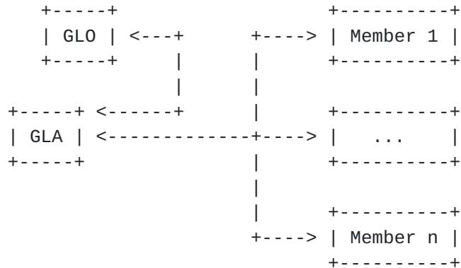
Figure 2 - Protocol Interactions
