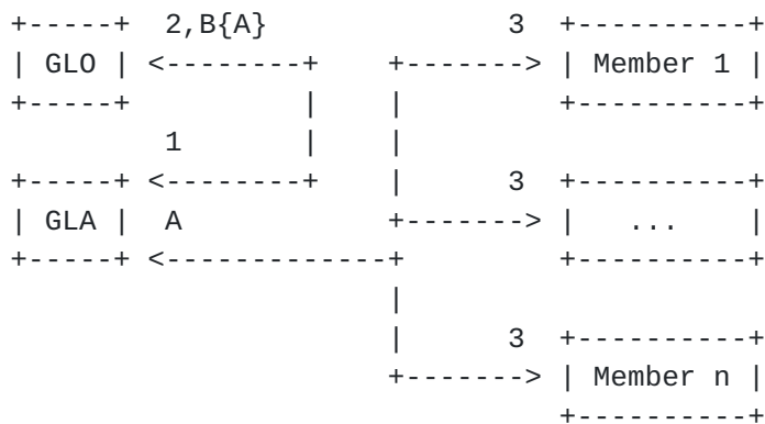
Figure 5 - Member Addition
