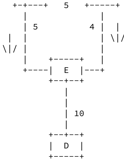
Figure 2: Link-Protecting Alternates Causing Loop on Node Failure
