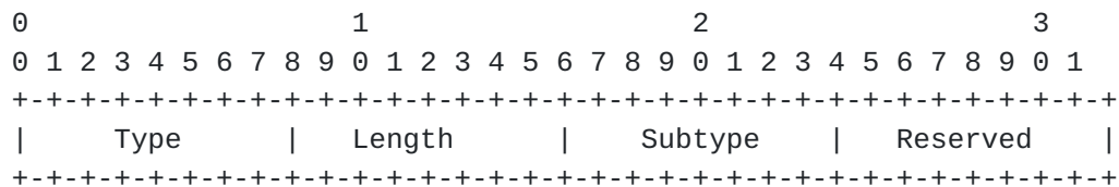
Figure 3: IPv6 Tunneling Mode Extension
