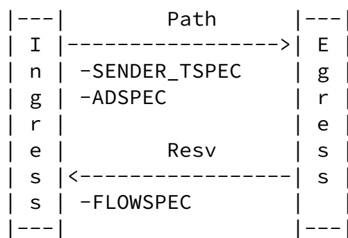
Figure 2: Asymmetric Bandwidth Bidirectional LSPs Using ADSPEC Object
