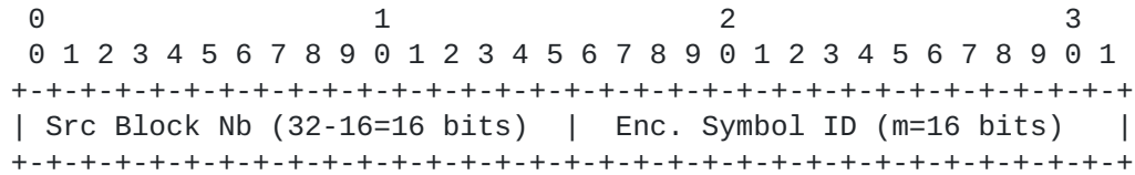
Figure 2: FEC Payload ID Encoding Format for m = 16
