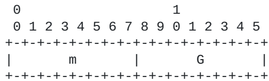
Figure 4: FEC OTI Scheme Specific Information To Be Included in the FDT Instance
