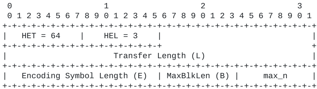
Figure 6: EXT_FTI Header Format with FEC Encoding ID 5
