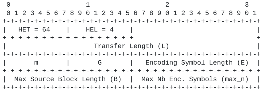
Figure 3: EXT_FTI Header Format
