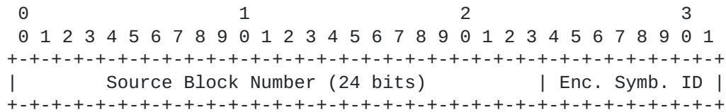
Figure 5: FEC Payload ID Encoding Format with FEC Encoding ID 5
