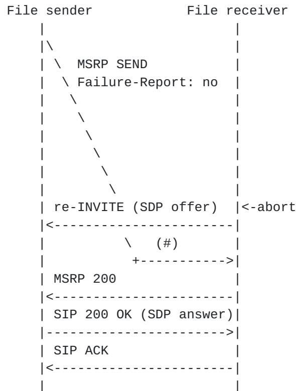
Figure 6: File receiver aborts an ongoing file transfer. Failure-Report set to "no" in MSRP
