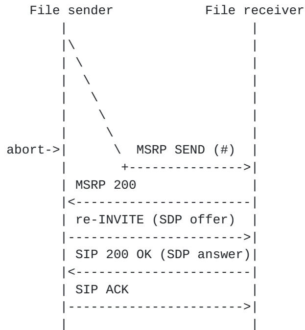
Figure 4: File sender aborts an ongoing file transfer
