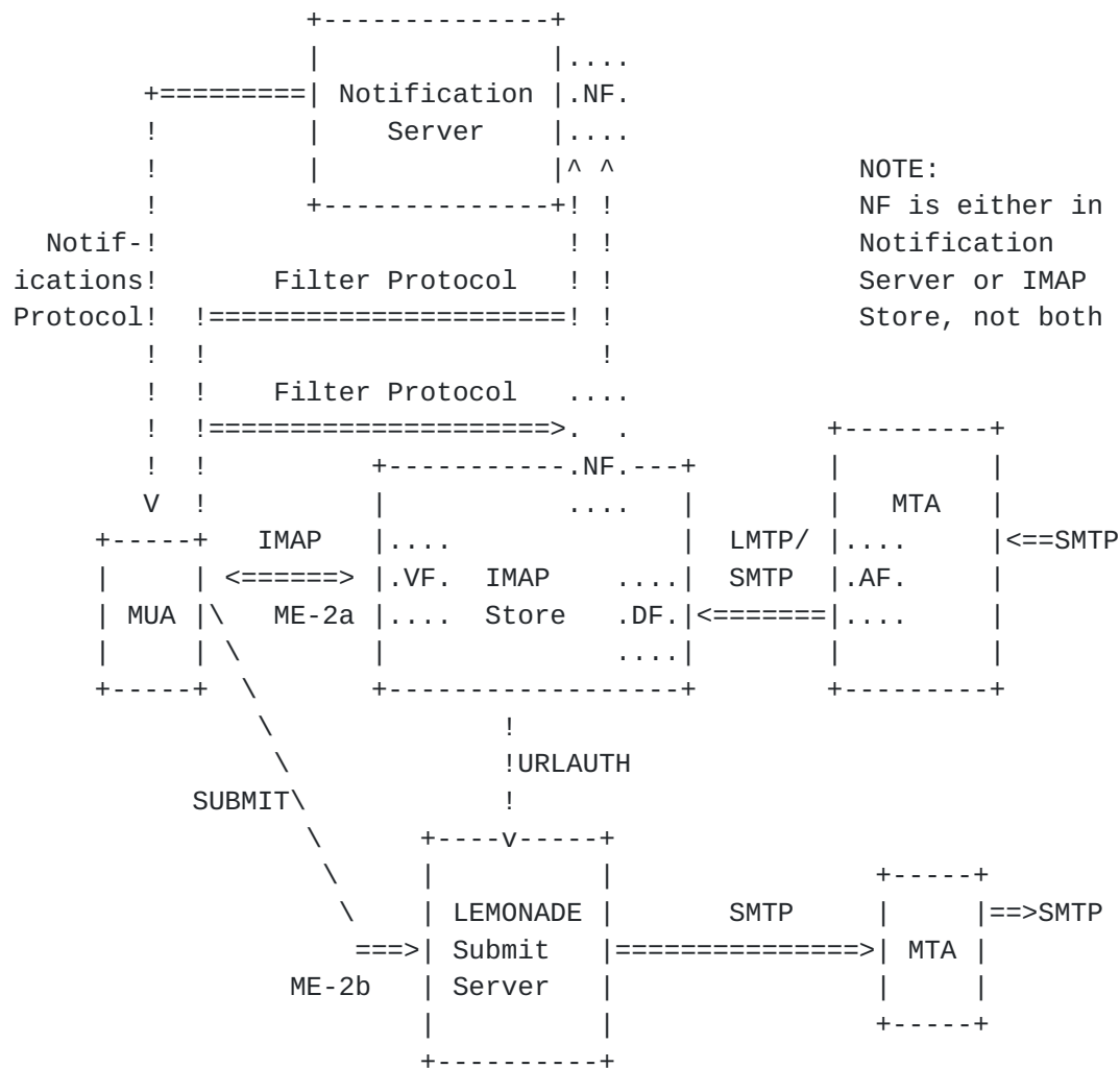
Figure 1: Filtering Mechanism Defined in Lemonade Profile Architecture
