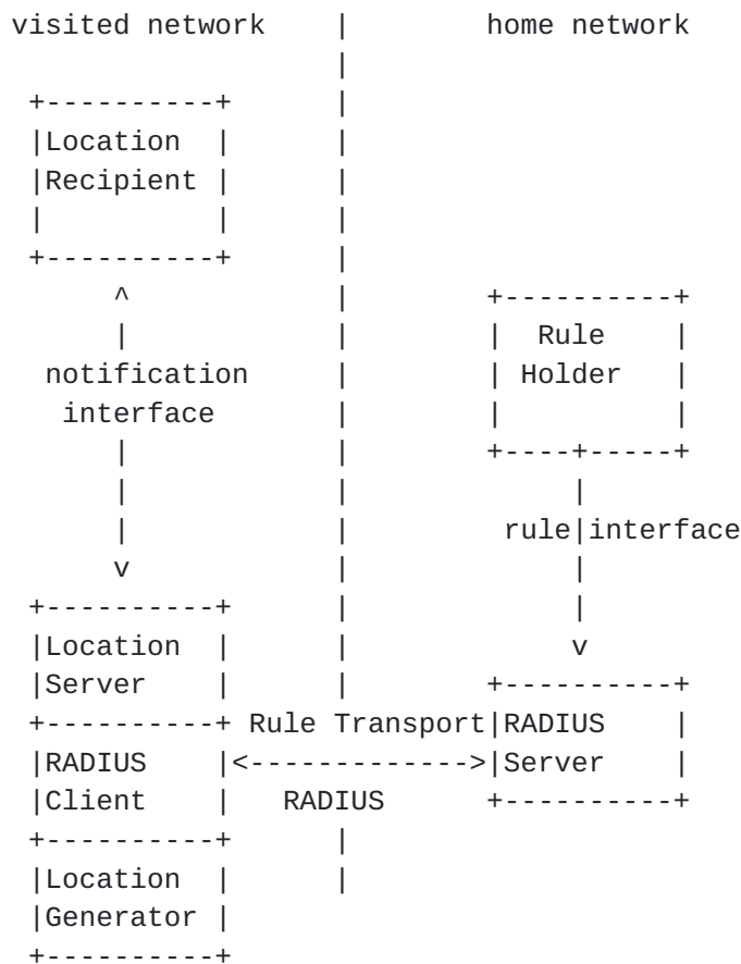
Figure 9: Location Server at the Visited Network
