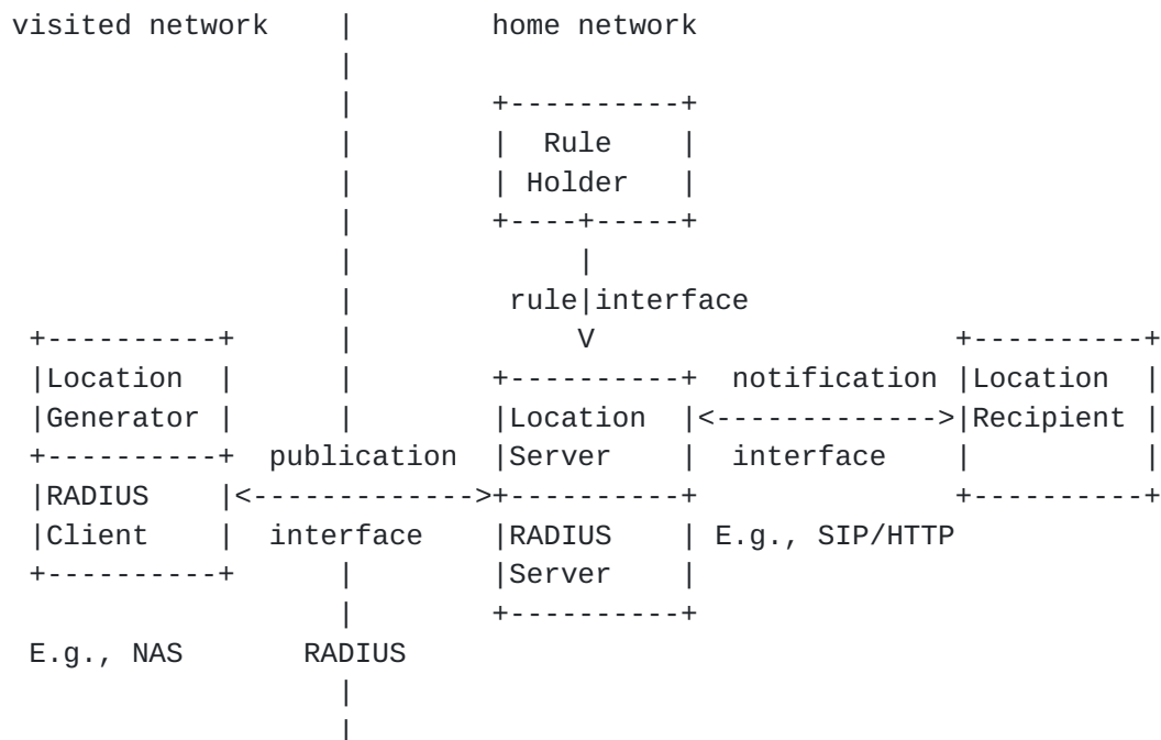
Figure 8: Location Server at the Home Network
