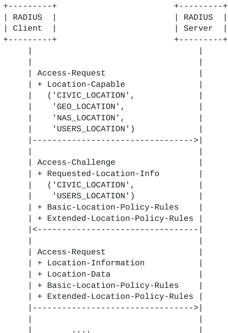
Figure 6: RADIUS Server Requesting Location Information
