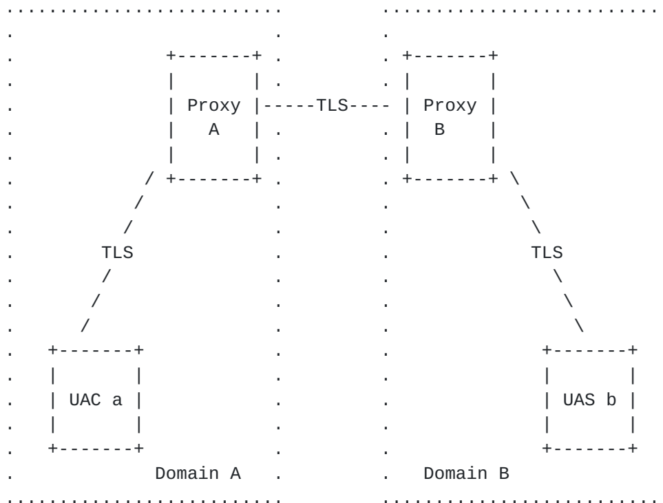
SIP trapezoid without last-hop exception
