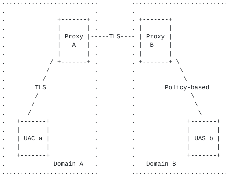
SIP trapezoid with last-hop exception
