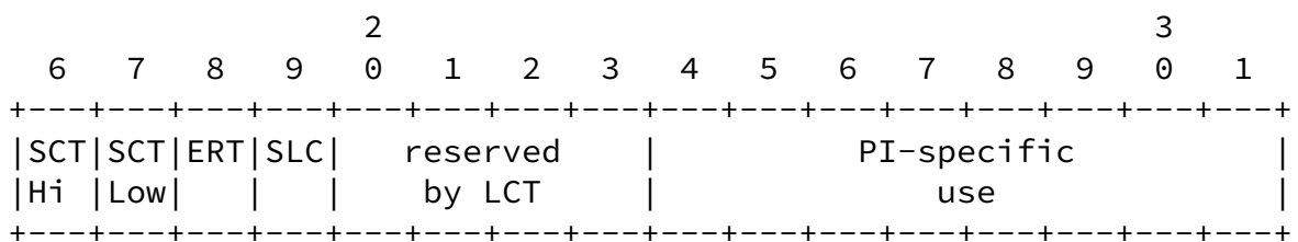
Figure 4: "Use" bit field format
