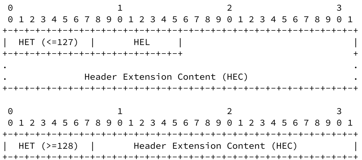
Figure 2: Format of additional headers
