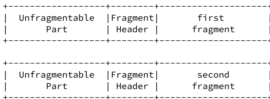
Figure 2: Fragmented IPv6 Packet
