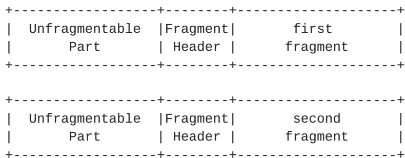
Figure 2: Fragmented IPv6 Packet
