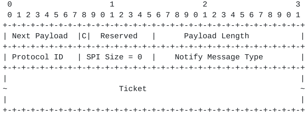
Figure 7: TICKET_OPAQUE Notify Payload
