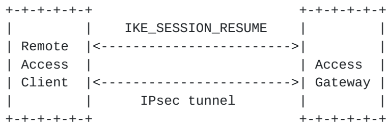
Figure 1: Resuming a Session with a Remote Access Gateway
