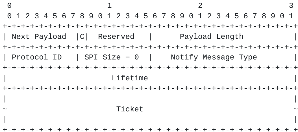
Figure 6: TICKET_LT_OPAQUE Notify Payload
