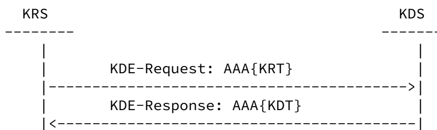
Figure 2: KDE Message Flow
