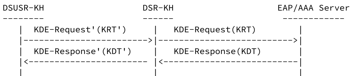
Figure 3: Combined Message Exchange
