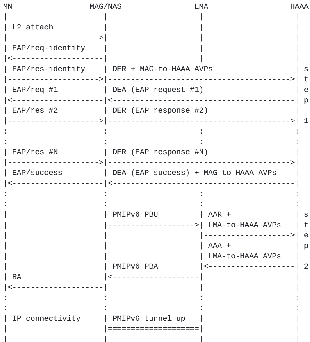
Figure 4: MAG and LMA Signaling Interaction with AAA Server during PMIPv6 Bootstrapping
