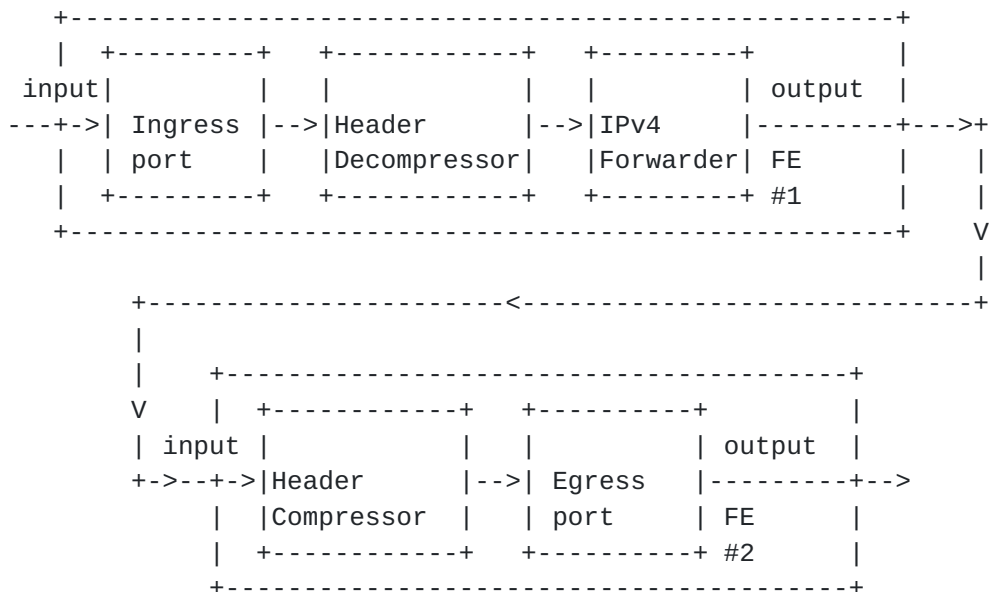
Figure 13: An example of two FEs connected together.
