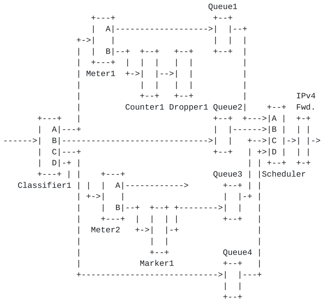
Figure 11: Another LFB topology as configured by the CE and accepted by the FE.
