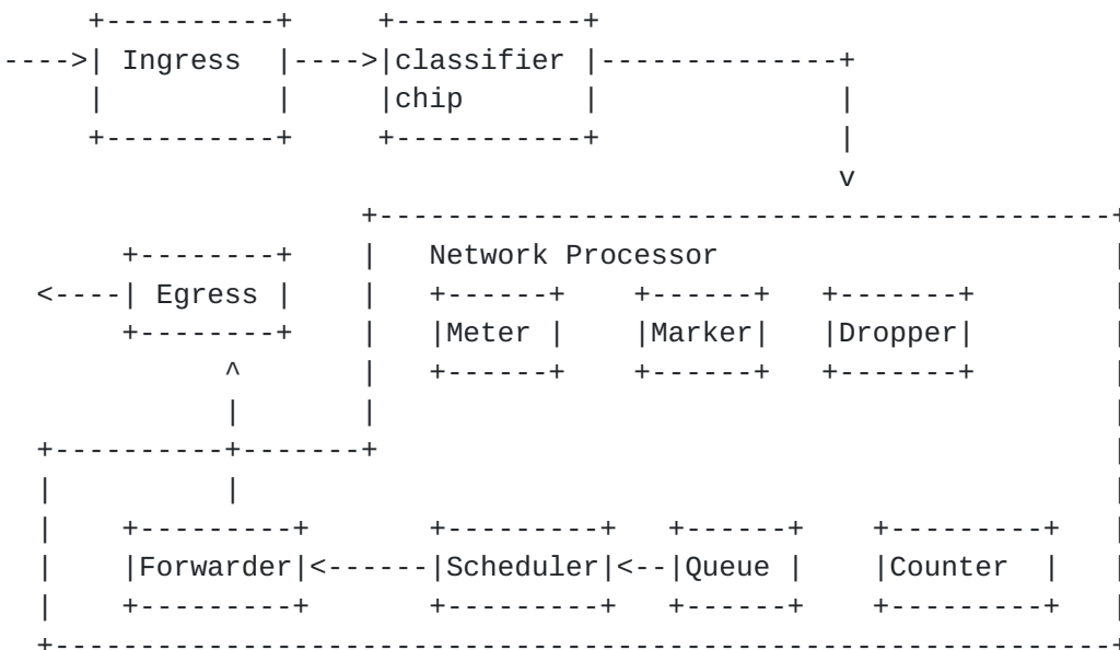
Figure 9: The capability of an FE as reported to the CE.
