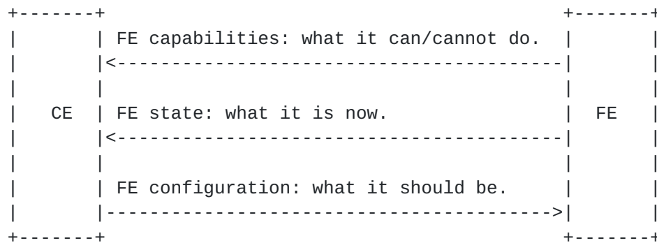
Figure 1: Illustration of FE capabilities, state, and configuration exchange in the context of CE-FE communication via ForCES.
