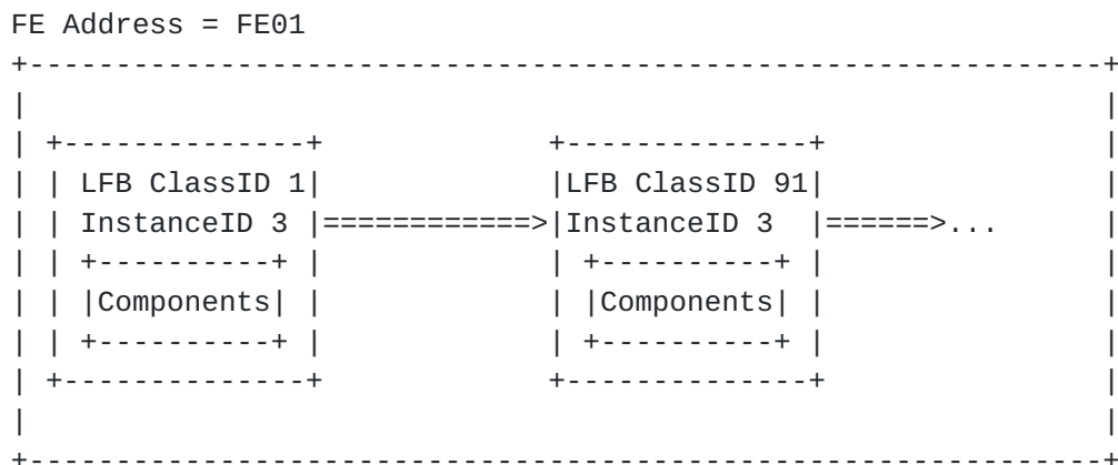
Figure 5: FE entity hierarchy.
