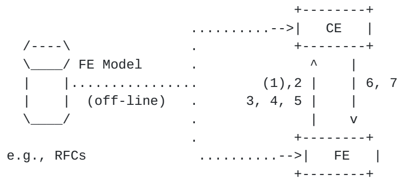
Figure 12: Relationship between the FE model and the ForCES protocol messages, where (1) is part of the ForCES base protocol, and the rest are defined by the FE model.
