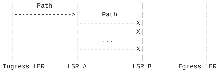
Figure 2: MP2CP - Path Msg and Communication Failure (Reliable Delivery)
