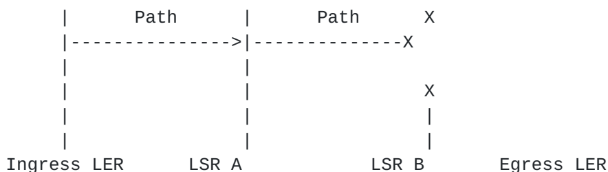
Figure 10: Case I - Path Message and Node Down
