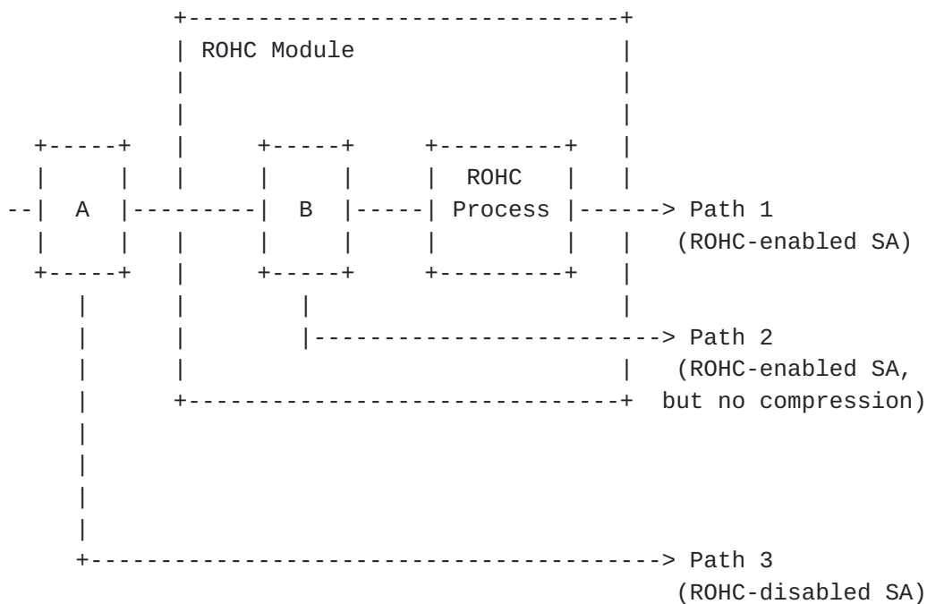
Figure 2. Integration of ROHC with IPsec
