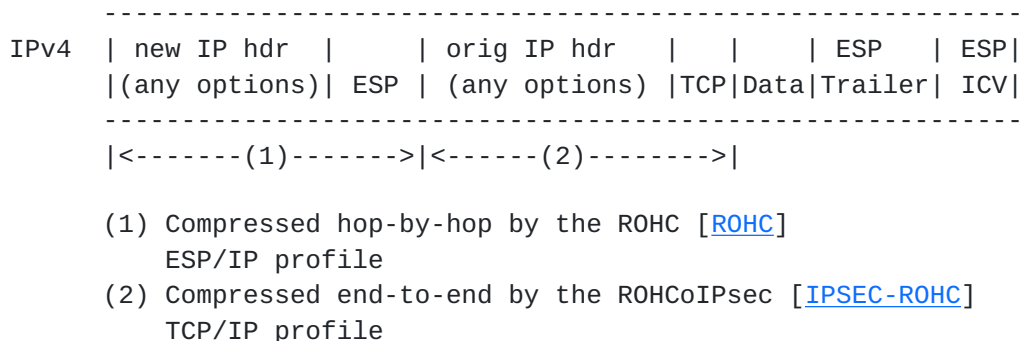
Figure 1. Applicability of hop-by-hop ROHC and ROHCoIPsec on an IPv4 ESP-processed packet.
