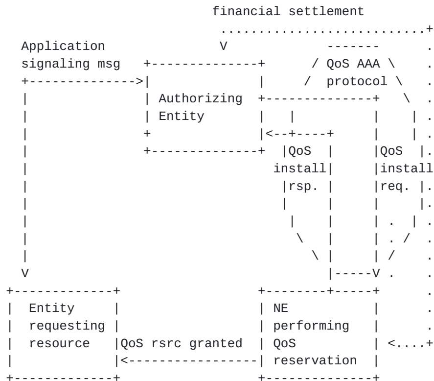
Figure 5: Scheme for Push Mode
