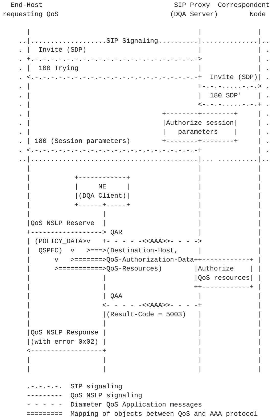
Figure 13: QoS Authorization Example - Pull Mode (Failure Case)
