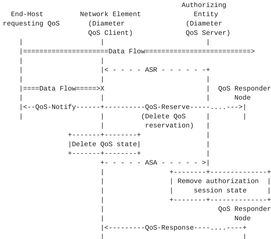
Figure 11: Server-Side Initiated Session Termination
