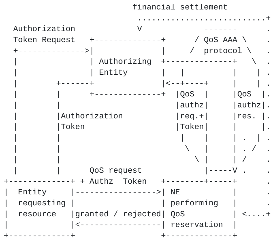
Figure 4: Token-Based Three-Party Scheme
