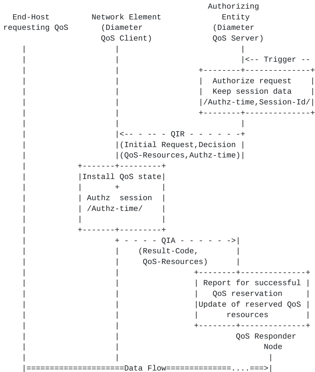
Figure 7: Initial QoS Request Authorization for Push Mode
