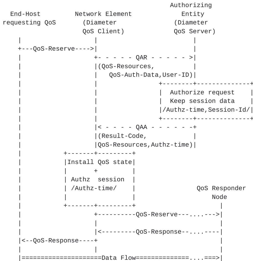
Figure 6: Initial QoS Request Authorization for Pull Mode
