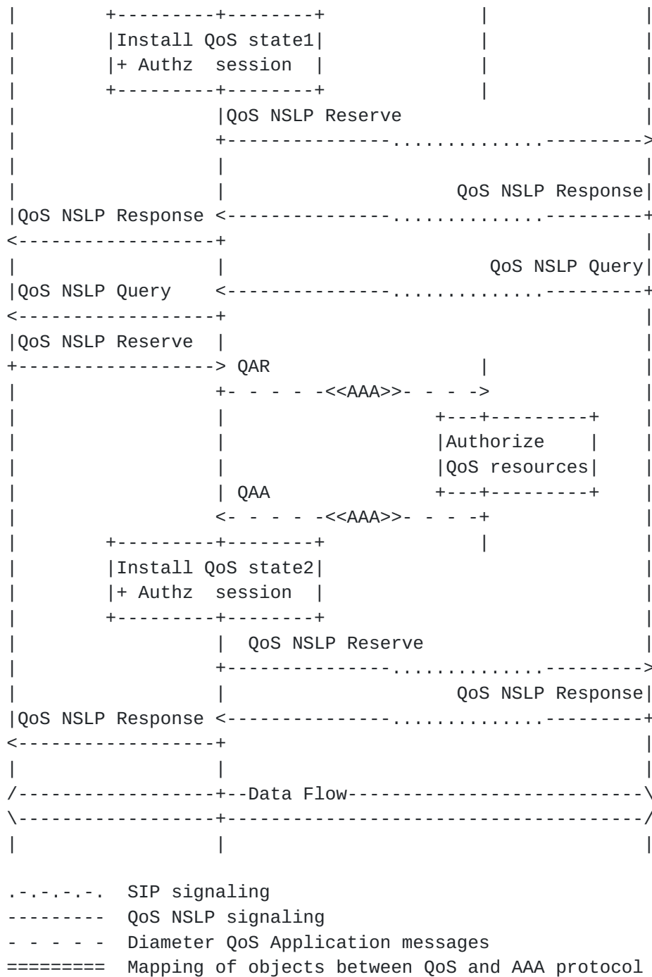
Figure 12: QoS Authorization Example - Pull Mode
