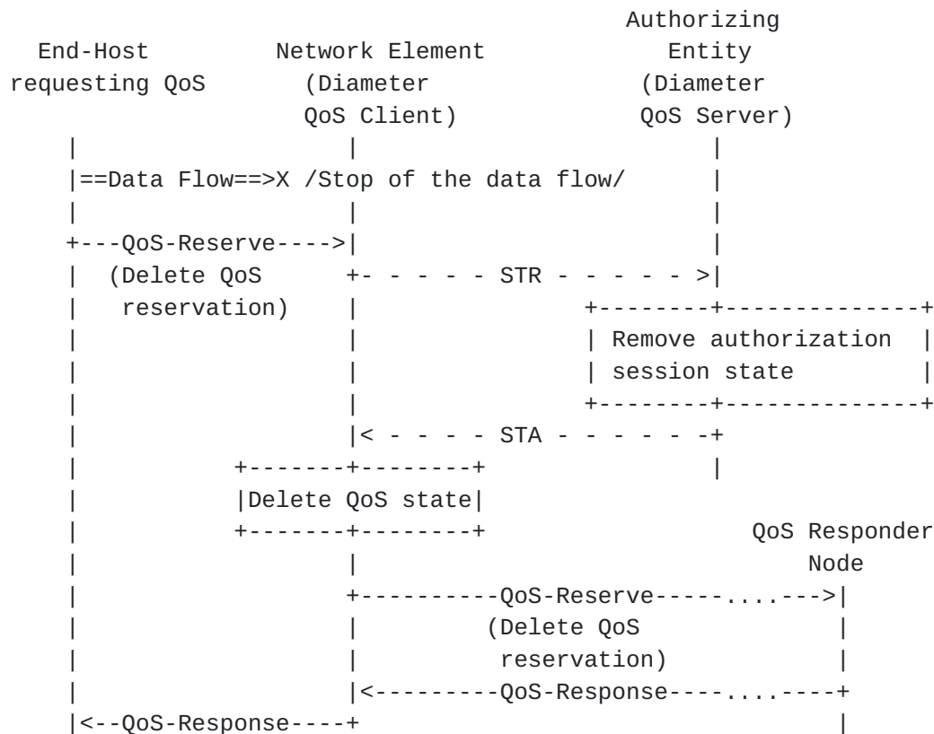
Figure 10: Client-Side Initiated Session Termination
