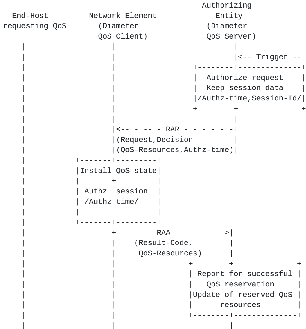
Figure 9: Server-Side Initiated QoS Re-Authorization
