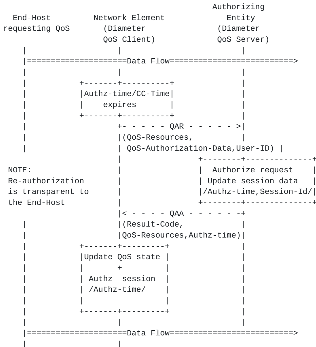
Figure 8: Client-side Initiated QoS Re-Authorization
