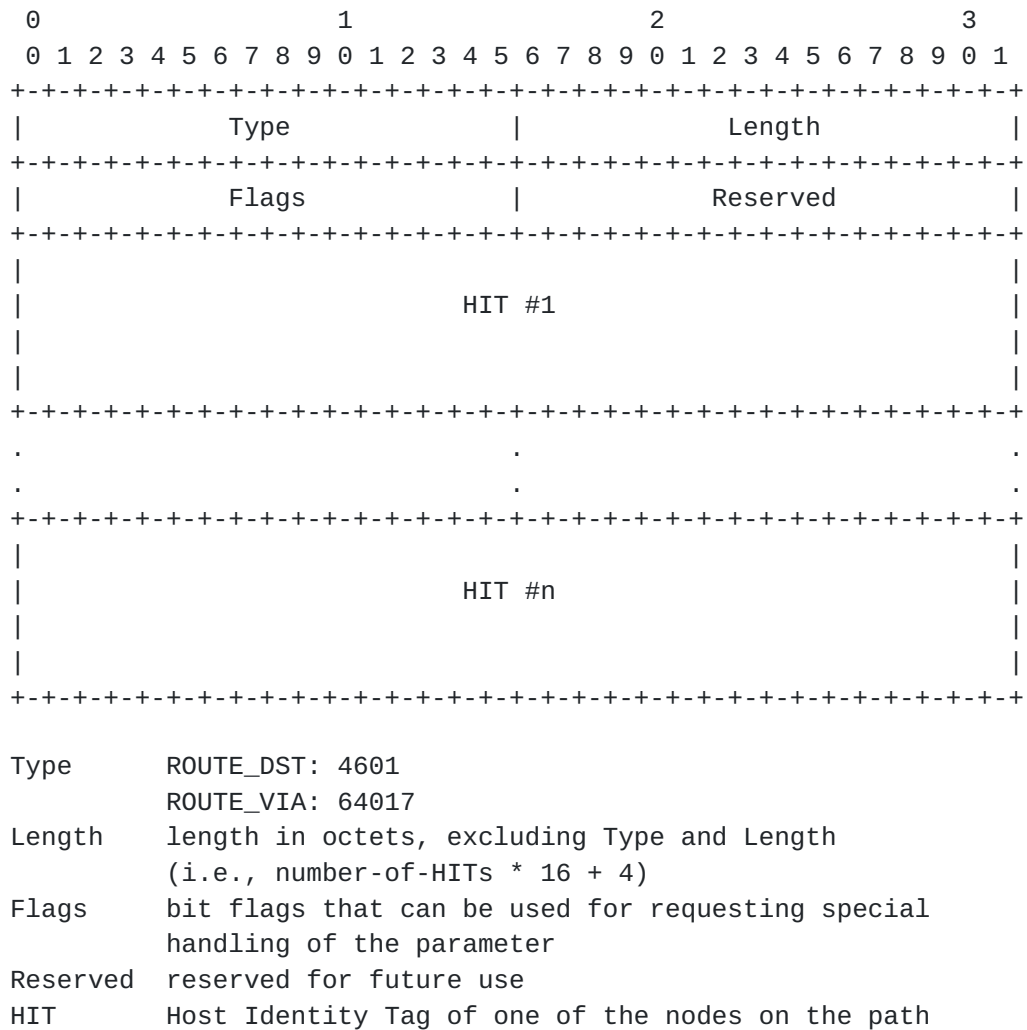
Figure 1. Format of the ROUTE_VIA and ROUTE_DST Parameters
