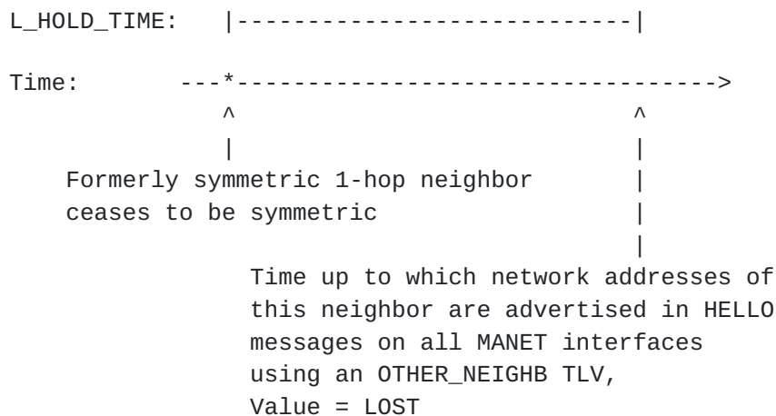
Figure 10: HELLO Message Generation: Advertisement of Formerly Symmetric 1-Hop Neighbor on Any MANET Interface as Lost
