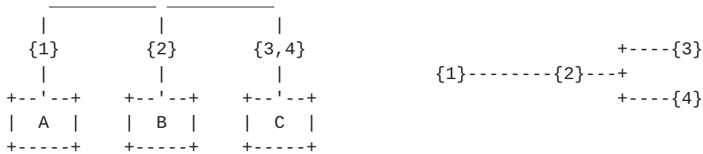
Figure 14: Single Interfaces, with 2-Hop Neighbor C Having Two Addresses (Left), and Corresponding NHDP Representation (Right)
