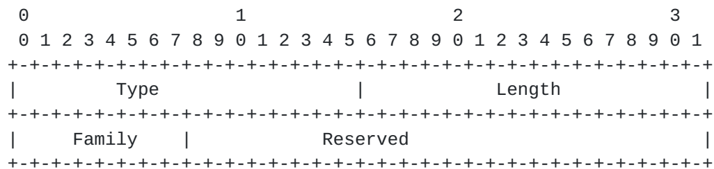
Figure 1: Format of REQUESTED-ADDRESS-FAMILY Attribute
