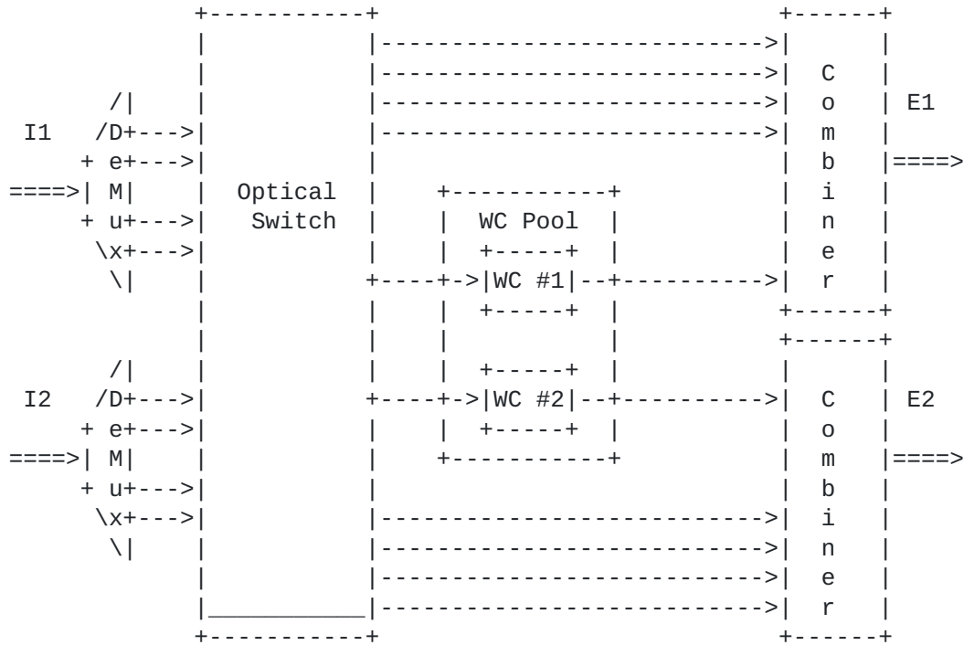
Figure 5. An optical switch featuring a shared per fiber wavelength converter pool architecture.
