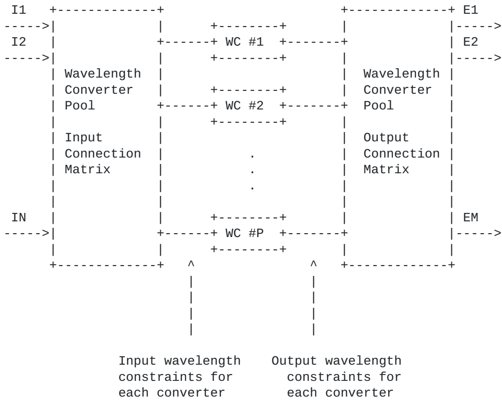
Figure 3. Schematic diagram of wavelength converter pool model.
