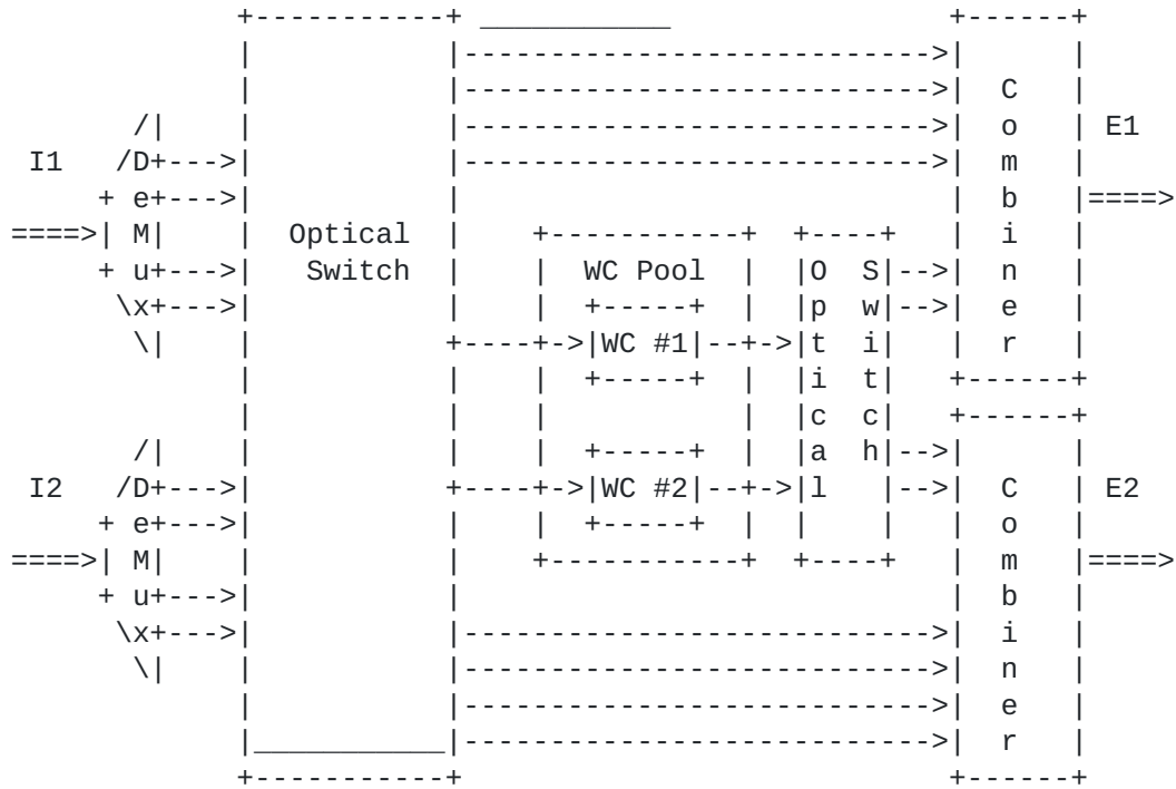
Figure 4. An optical switch featuring a shared per node wavelength converter pool architecture.
