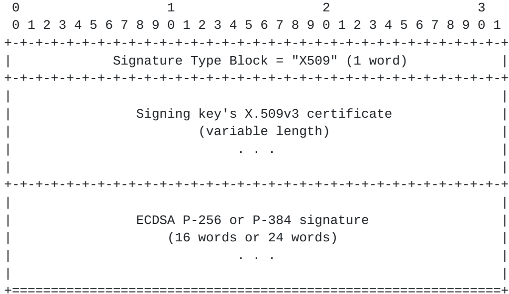
Figure 21: X.509v3 ECDSA Signature Format
