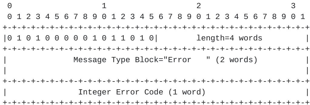
Figure 12: Error Message Format
