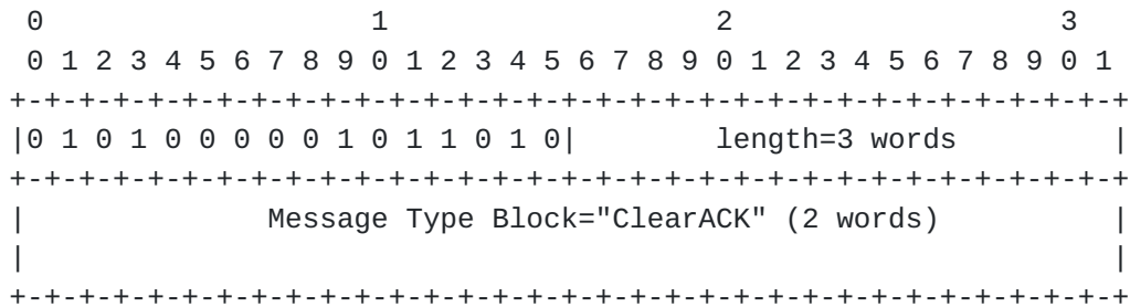
Figure 15: ClearACK Message Format
