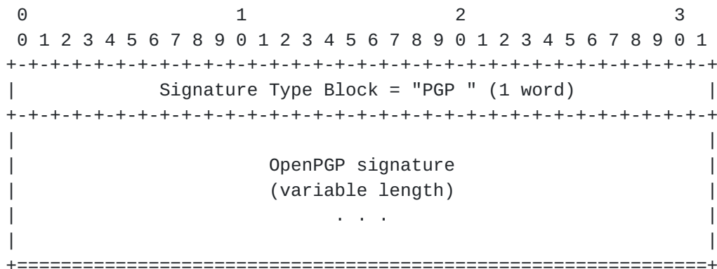
Figure 20: OpenPGP Signature Format
