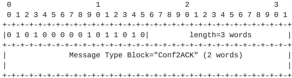
Figure 11: Conf2ACK Message Format
