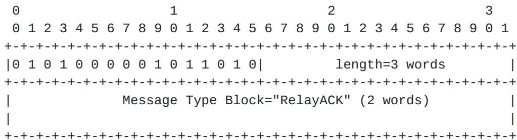
Figure 17: RelayACK Message Format
