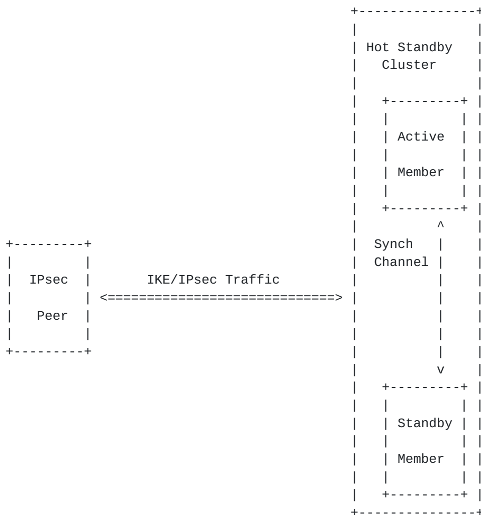
An IPsec Hot Standby Cluster
