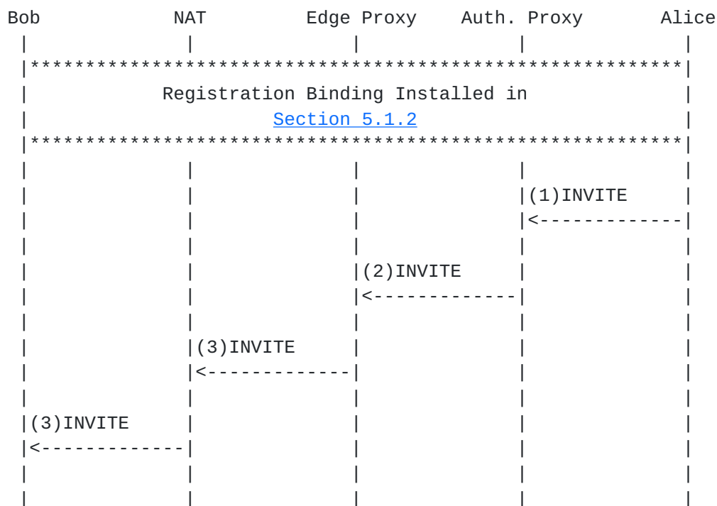
Figure 10: Registrar/Proxy Not Co-located
