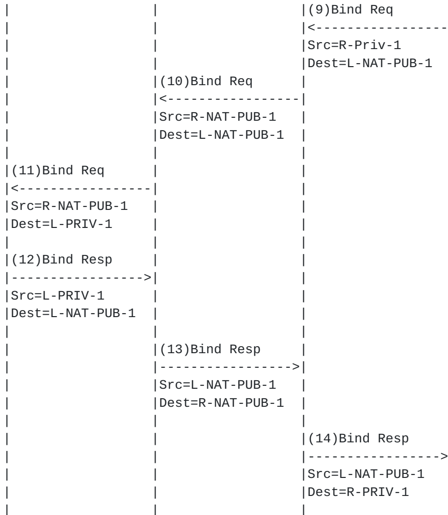
Figure 20: Single Address/Port-Dependent NAT - Success
