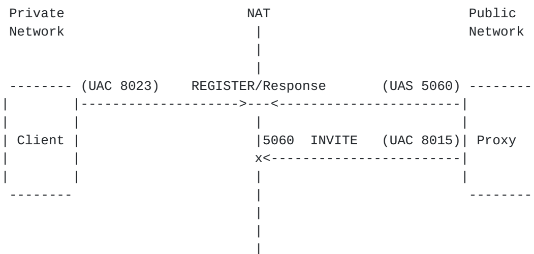
Figure 2: Failed Request
