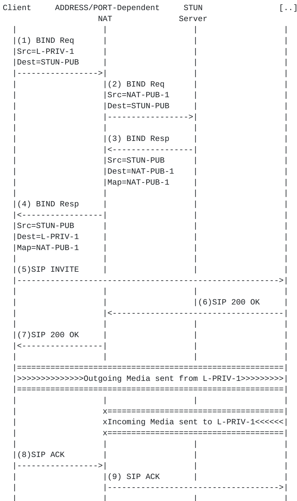
Figure 18: Address/Port-Dependent NAT with STUN - Failure
