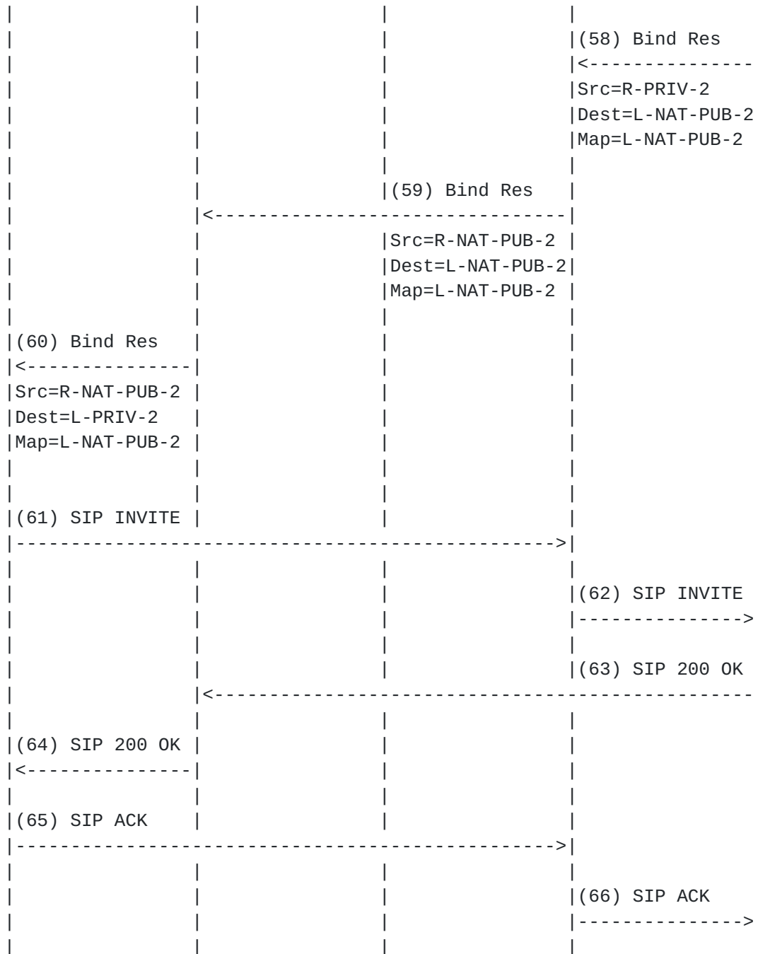
Figure 13: Endpoint-Independent NAT with ICE
