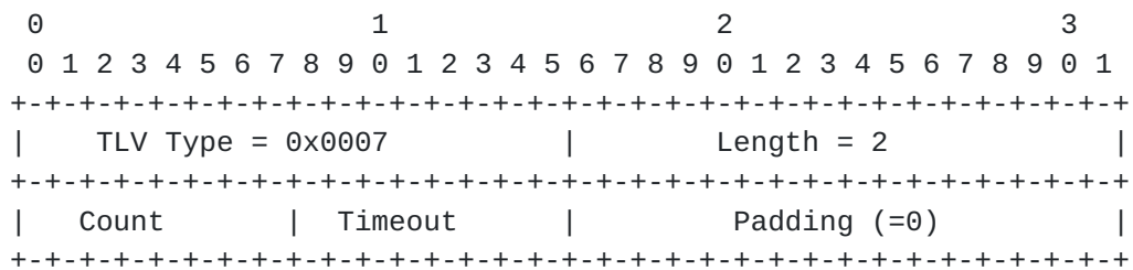
Figure 22: The OAM-Loopback-Test-Parameters TLV
