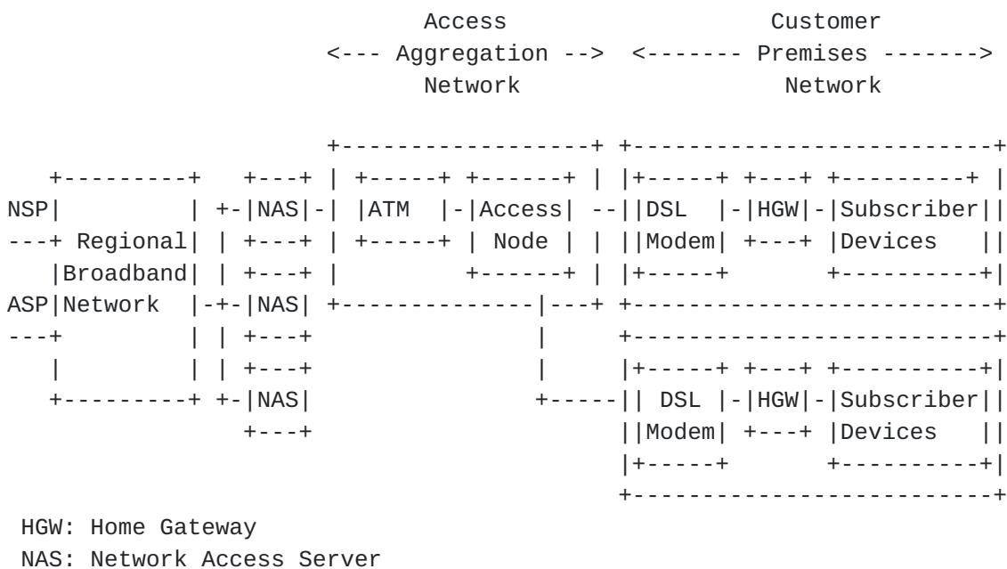
Figure 2: ATM Broadband Aggregation Topology
