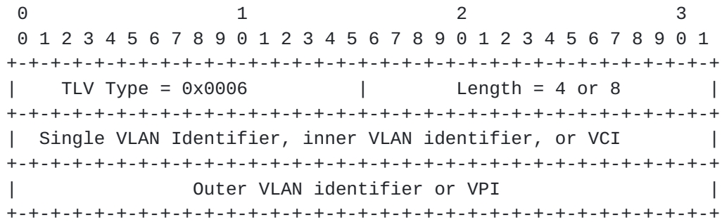
Figure 13: The Access-Aggregation-Circuit-ID-Binary TLV
