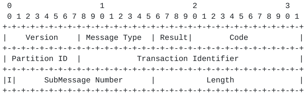
Figure 6: The Adjacency Update Message
