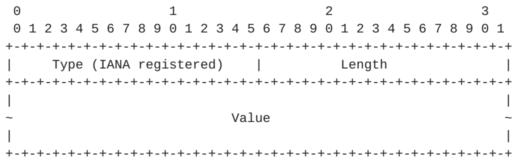
Figure 8: General TLV Format
