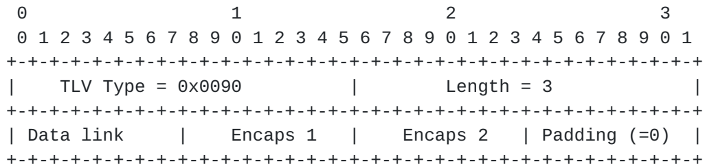
Figure 16: The Access-Loop-Encapsulation TLV
