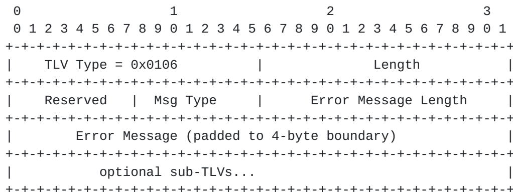
Figure 12: The Status-Info TLV
