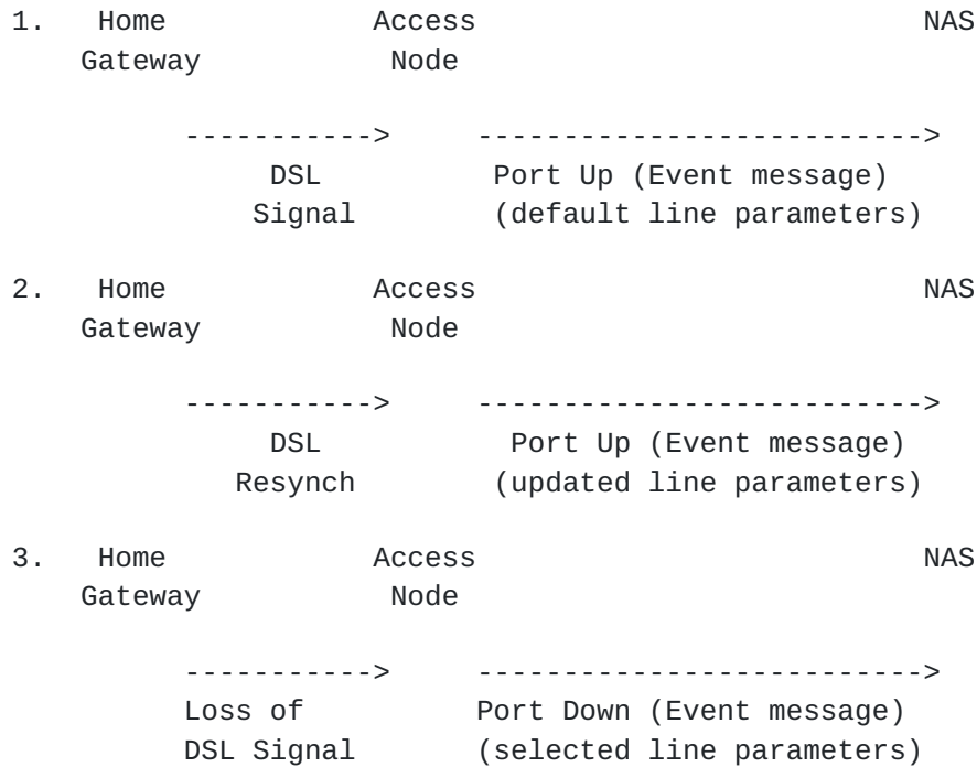
Figure 14: ANCP Message Flow for DSL Topology Discovery
