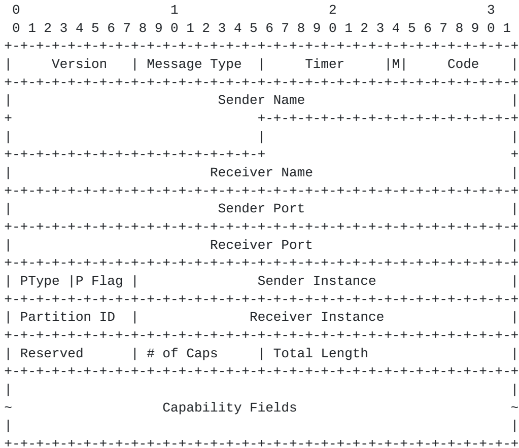
Figure 4: ANCP Adjacency Message Format
