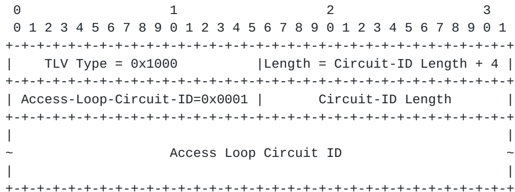
Figure 11: Example of Target TLV for Single Access Line
