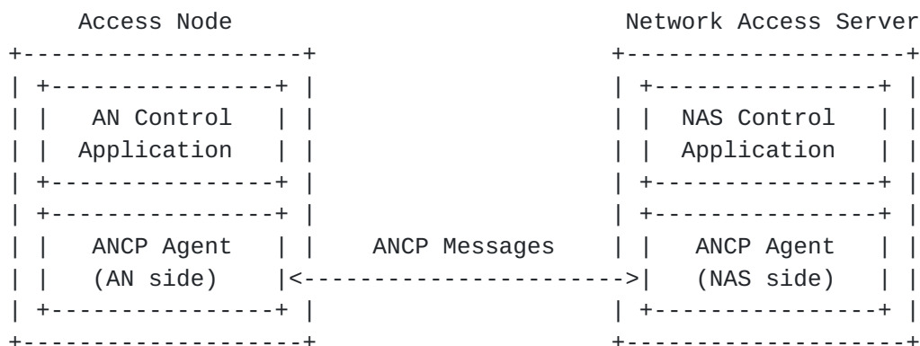
Figure 1: Architectural Context for the Access Node Control Protocol
