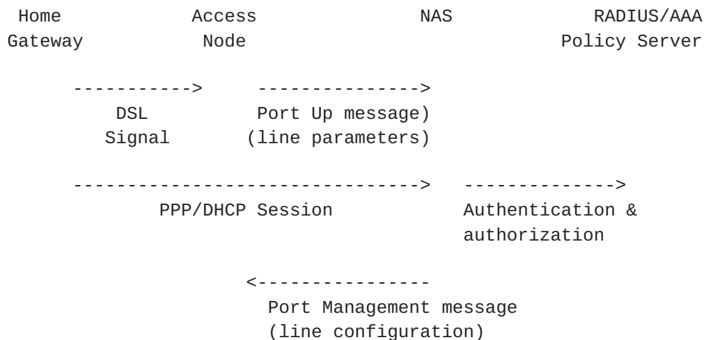
Figure 17: Message Flow - ANCP Mapping for Initial Line Configuration
