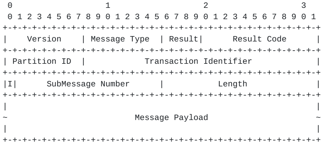
Figure 7: ANCP General Message Format
