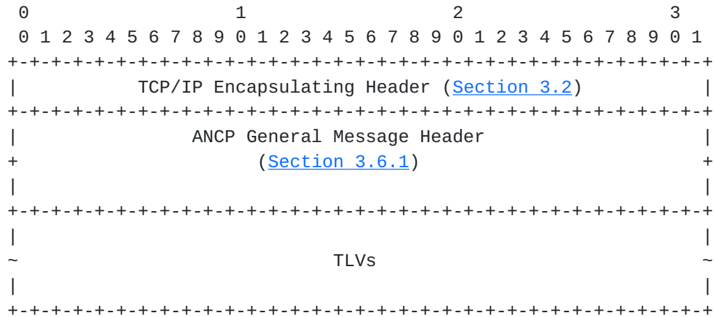
Figure 9: Format of the Provisioning Message
