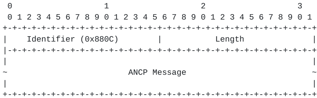
Figure 3: Encapsulation of ANCP Messages over TCP/IP
