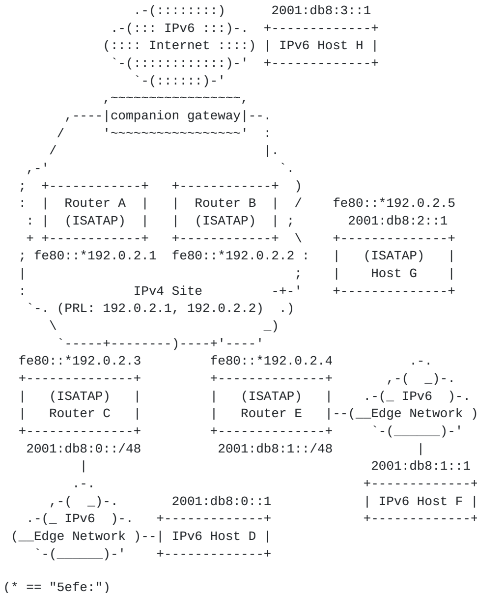
Figure 2: Reference ISATAP Network Topology
