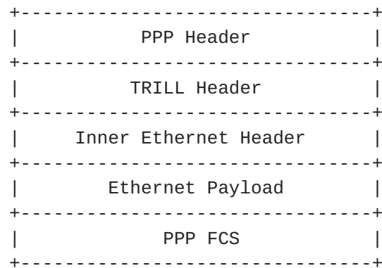
Figure 3: A PPP Encapsulated TRILL Frame
