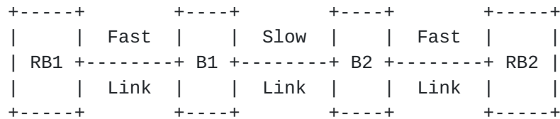
Figure 12: Link Cost of a Bridged Link
