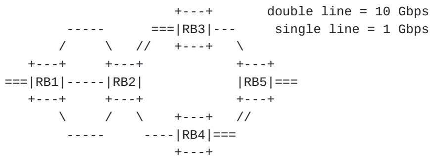
Figure 15: Known Unicast Multipath
