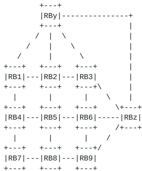
Figure 14: Multi-Destination Multipath
