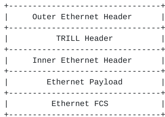
Figure 2: An Ethernet Encapsulated TRILL Frame
