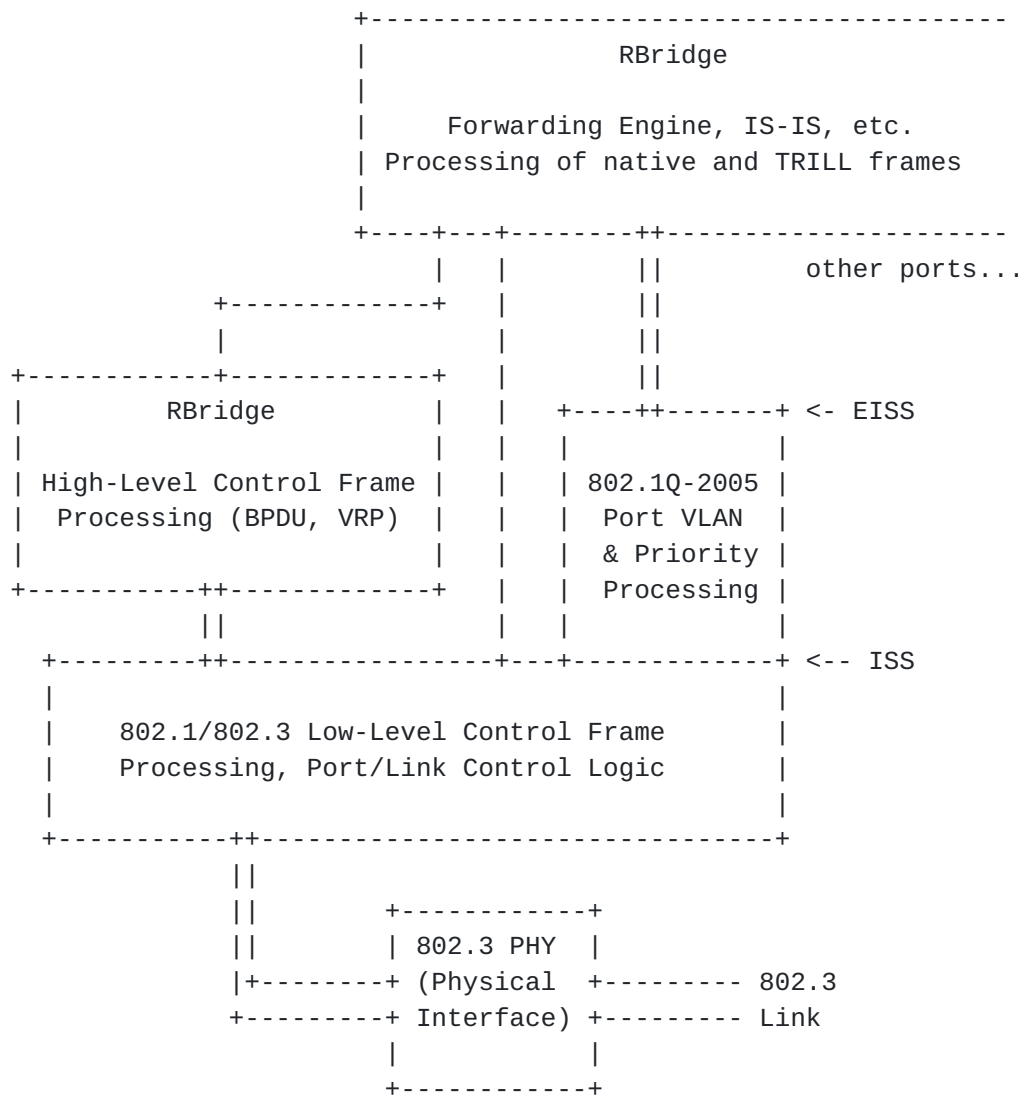
Figure 4: RBridge Port Model
