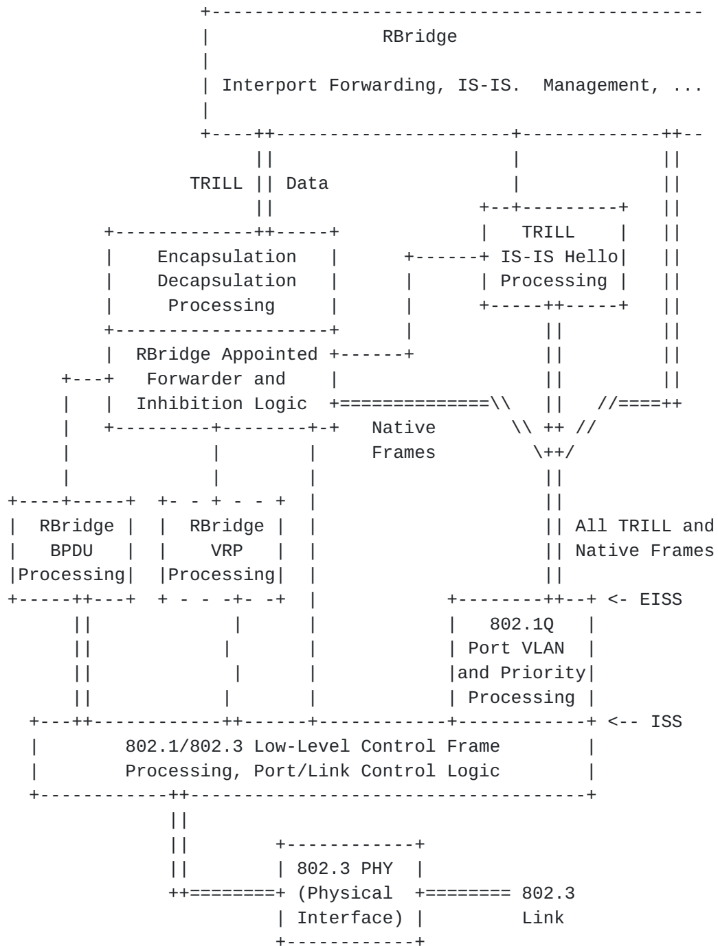
Figure 11: Detailed RBridge Port Model
