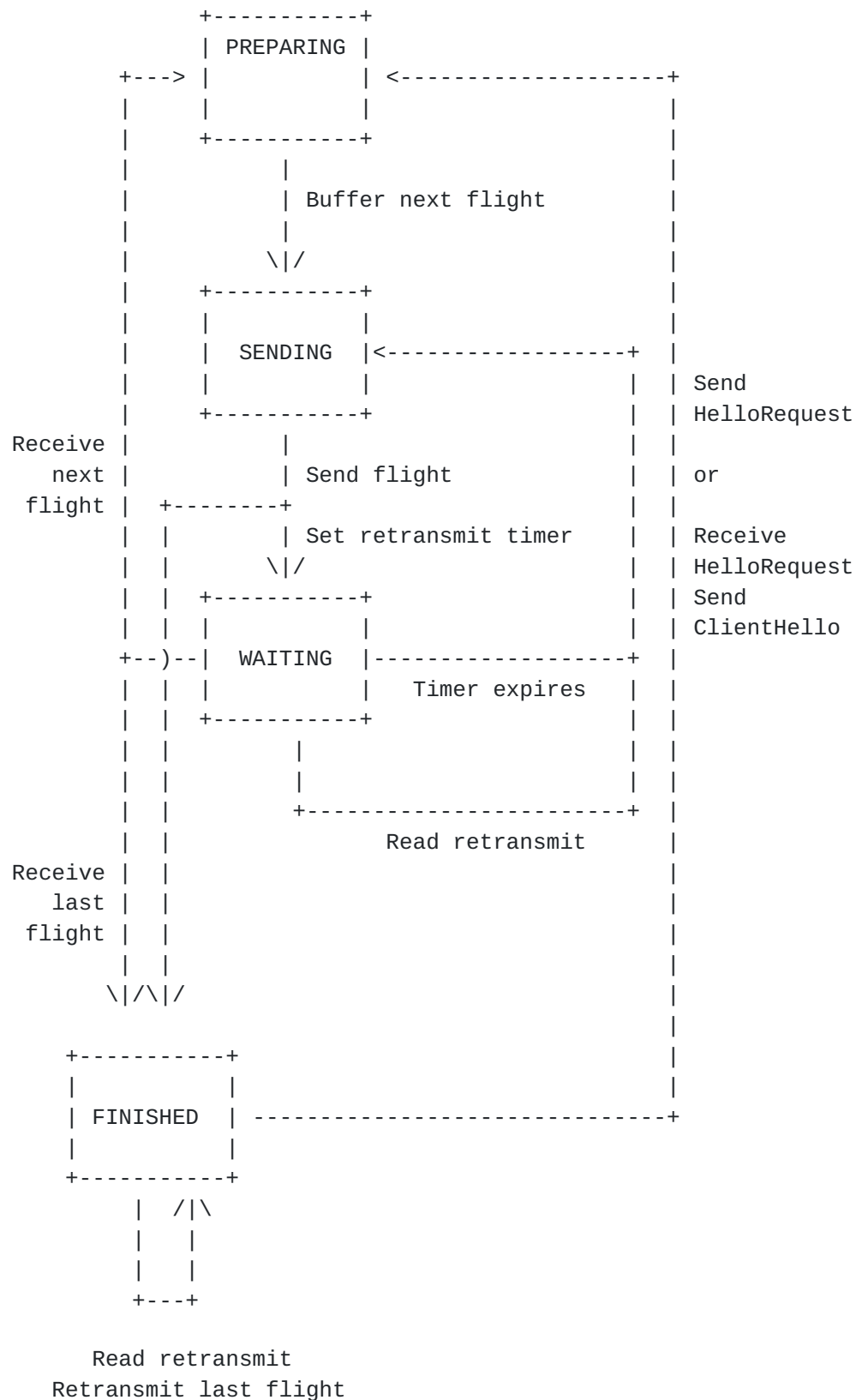
Figure 3. DTLS Timeout and Retransmission State Machine
