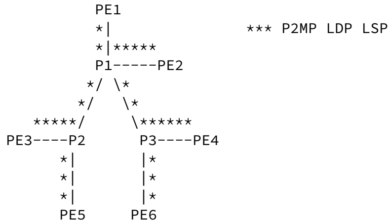
Figure 2: Attachment of PE5 and PE6.
