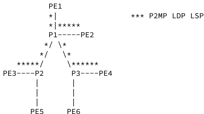
Figure 1: P2MP LSP from PE1 to PE2, PE3, PE4.
