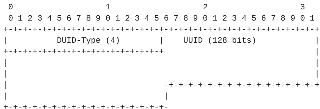
Figure 1: DUID-UUID Format
