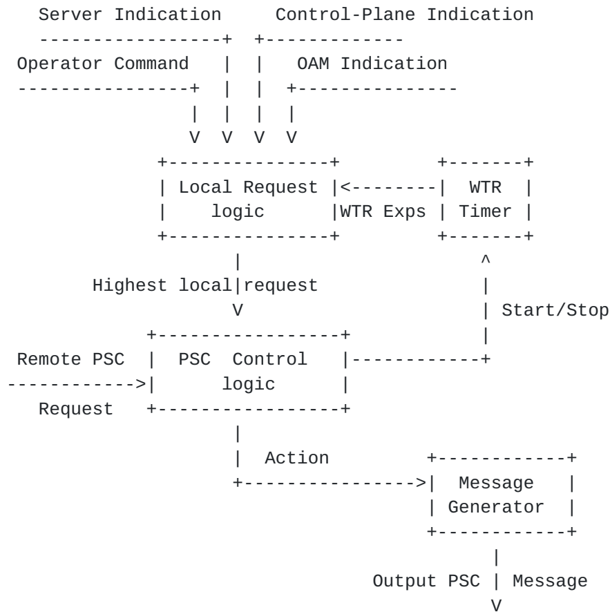
Figure 1: Protection State Control Logic
