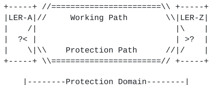
Figure 3: Protection Domain
