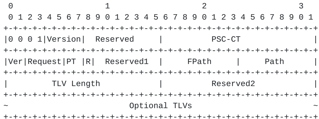
Figure 2: Format of PSC Packet with a G-ACh Header
