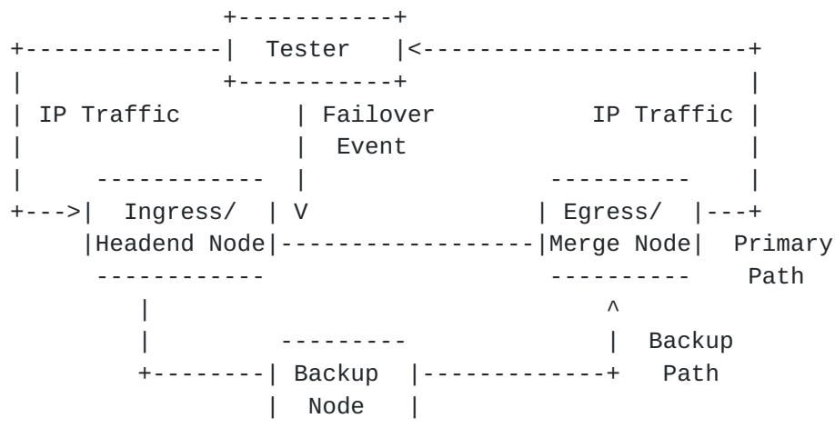
Figure 1. System Under Test (SUT) for Sub-IP Link Protection
