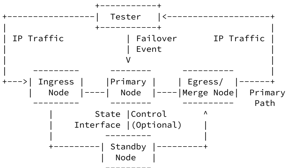
Figure 5. System Under Test (SUT) for Sub-IP Redundant Node Protection
