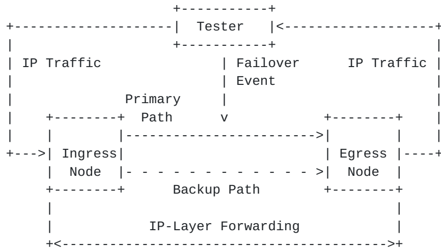
Figure 4. System Under Test (SUT) for Sub-IP Local Link Protection
