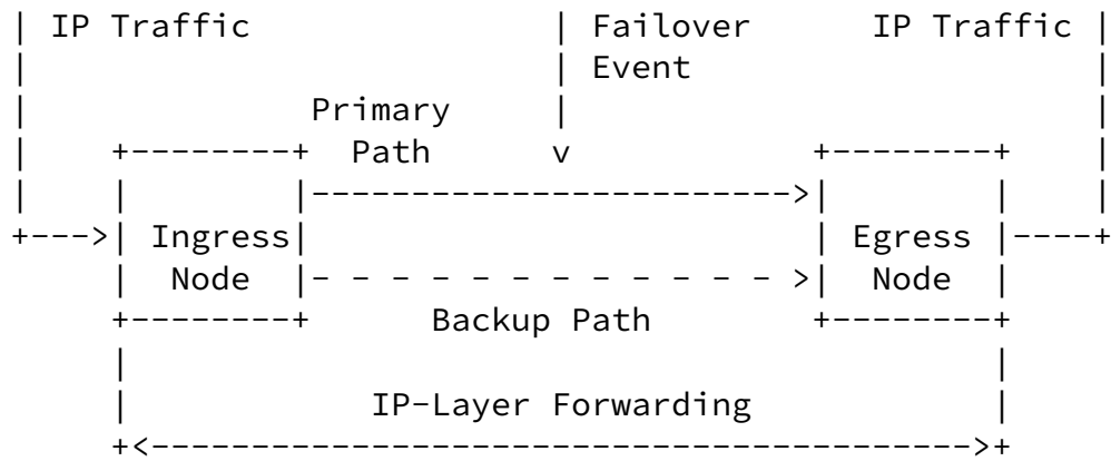
Figure 4. System Under Test (SUT) for Sub-IP Local Link Protection
