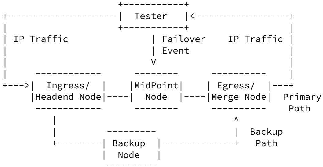
Figure 2. System Under Test (SUT) for Sub-IP Node Protection
