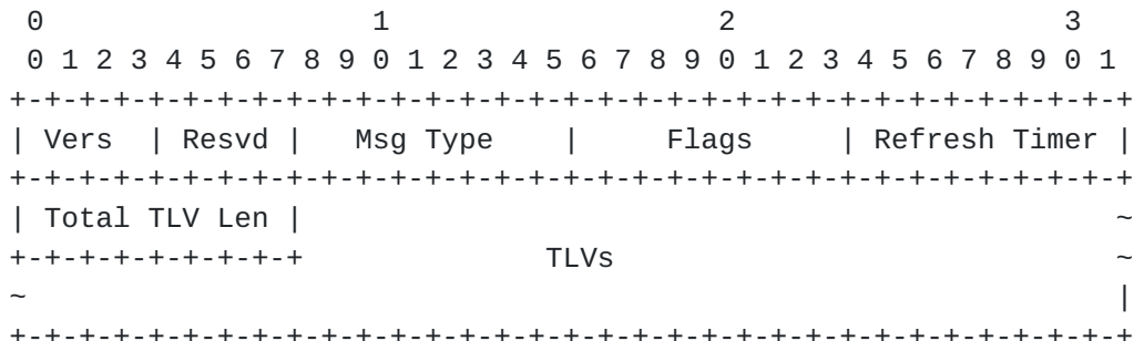
Figure 2: MPLS Fault OAM Message Format
