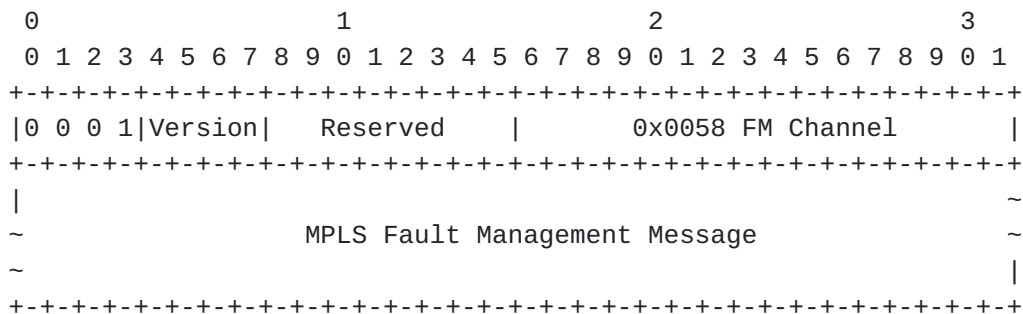
Figure 1: ACH Indication of the MPLS Fault Management Channel
