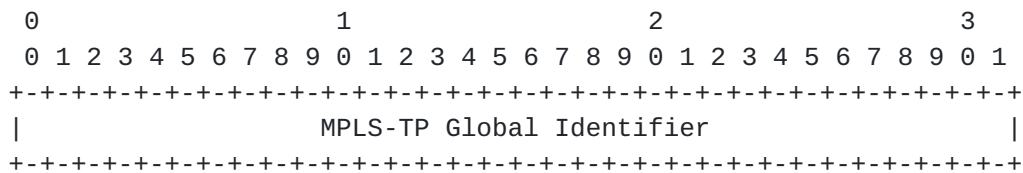
Figure 6: Global Identifier TLV Format
