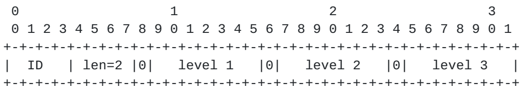
Figure 2: Sample Audio Level Encoding Using the One-Byte Header Format
