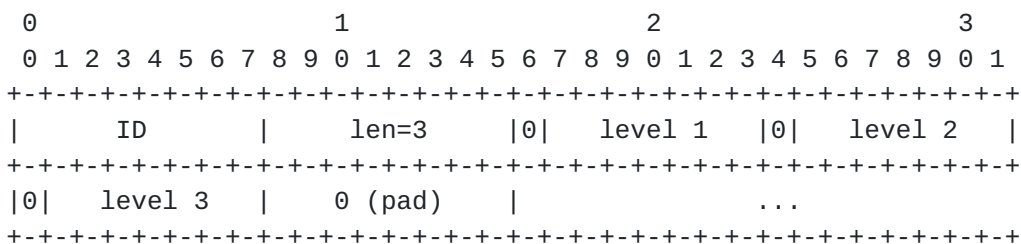
Figure 3: Sample Audio Level Encoding Using the Two-Byte Header Format
