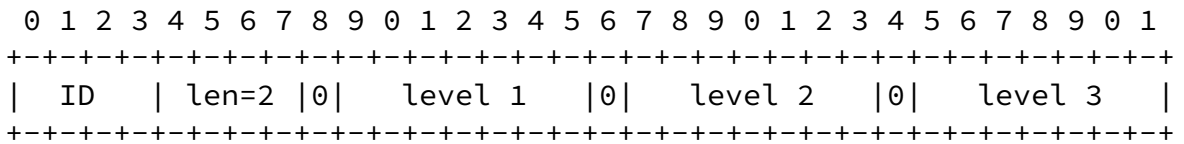
Figure 2: Sample Audio Level Encoding Using the One-Byte Header Format
