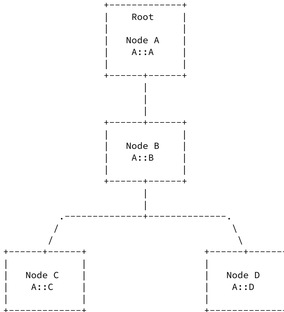
Figure 33: Storing Mode with Subnet-Wide Prefix
