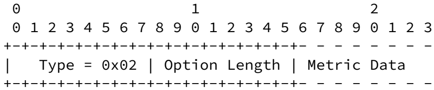
Figure 22: Format of the DAG Metric Container Option
