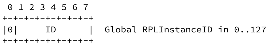
Figure 4: RPLInstanceID Field Format for Global Instances
