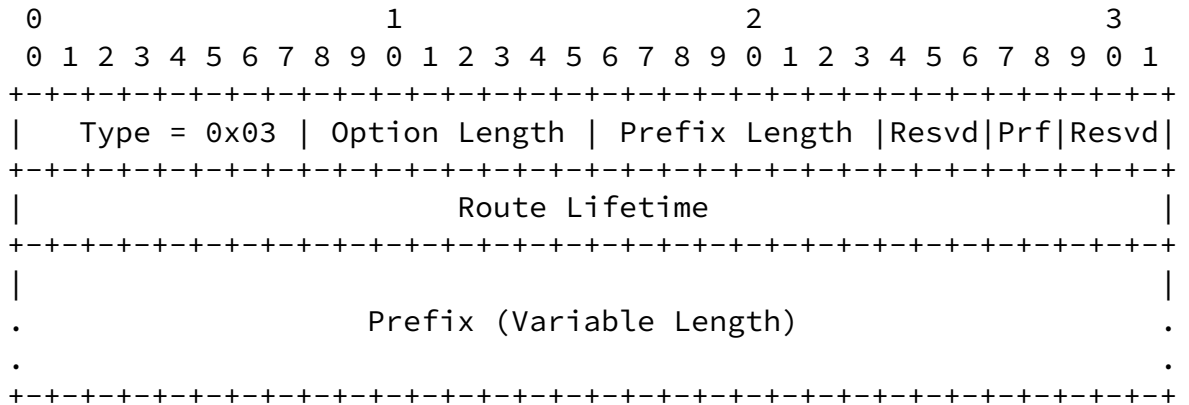
Figure 23: Format of the Route Information Option
