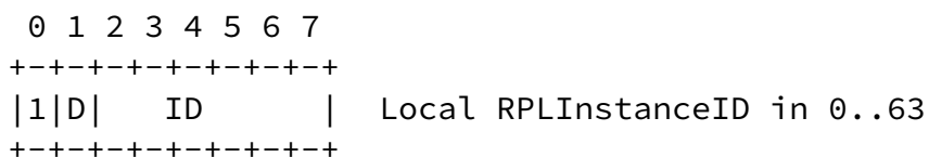
Figure 5: RPLInstanceID Field Format for Local Instances
