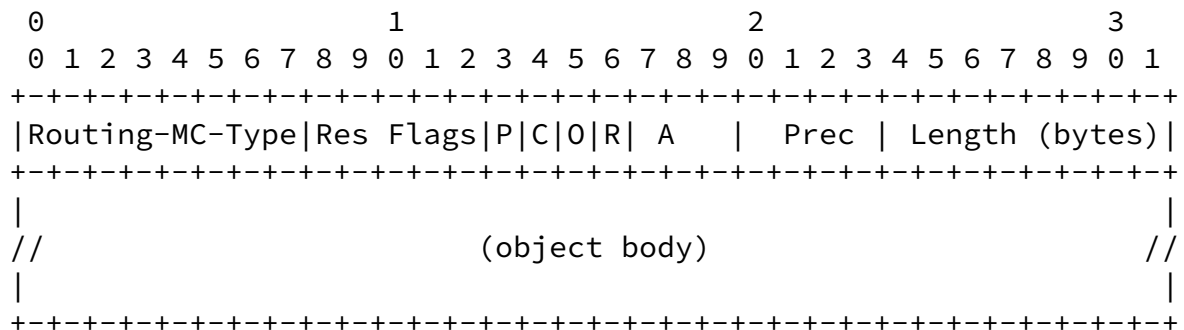
Figure 1: Routing Metric/Constraint Object Generic Format
