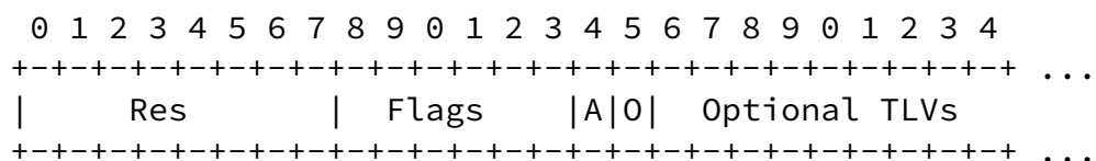
Figure 2: NSA Object Body Format
