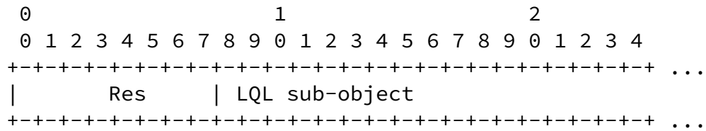
Figure 10: LQL Object Body Format
