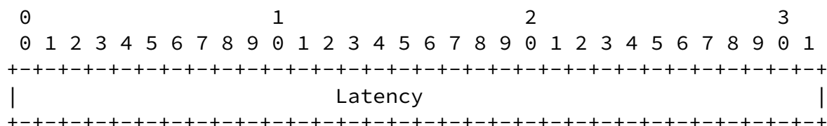
Figure 9: Latency Sub-Object Format
