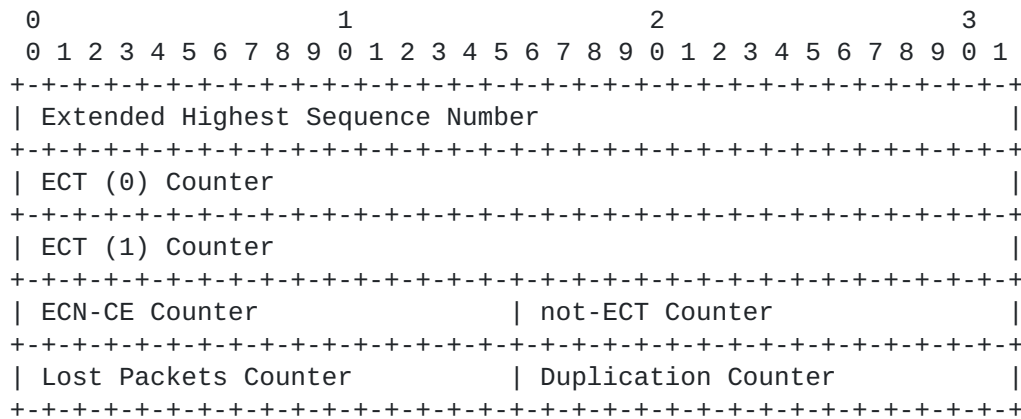
Figure 2: ECN Feedback Report Format
