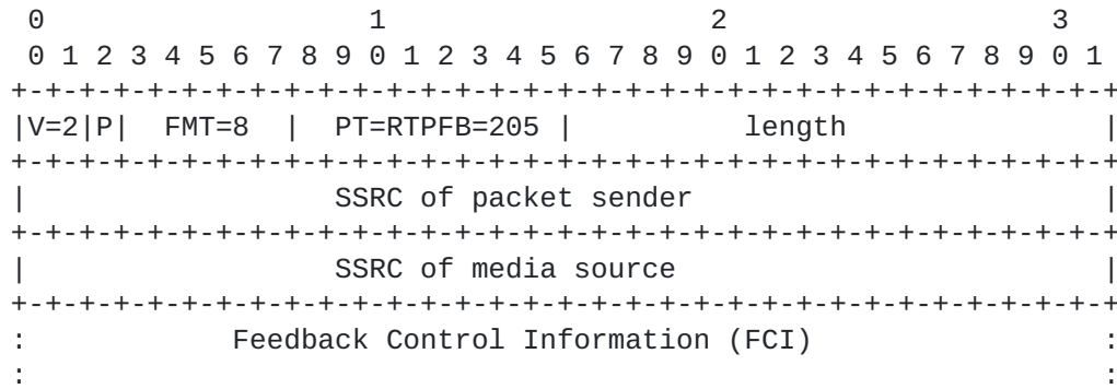
Figure 1: RTP/AVPF Common Packet Format for Feedback Messages
