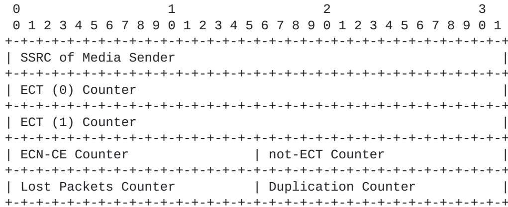
Figure 4: RTCP XR ECN Summary Report
