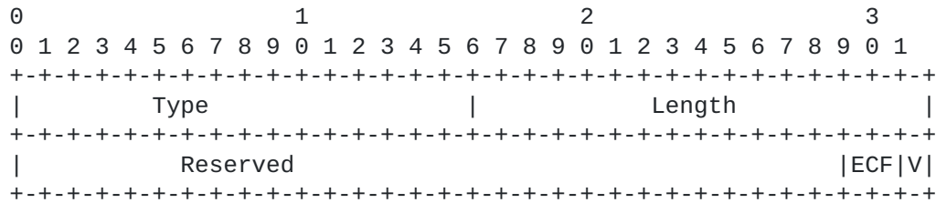
Figure 6: ECN-CHECK STUN Attribute
