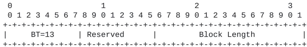
Figure 3: RTCP XR Report Header
